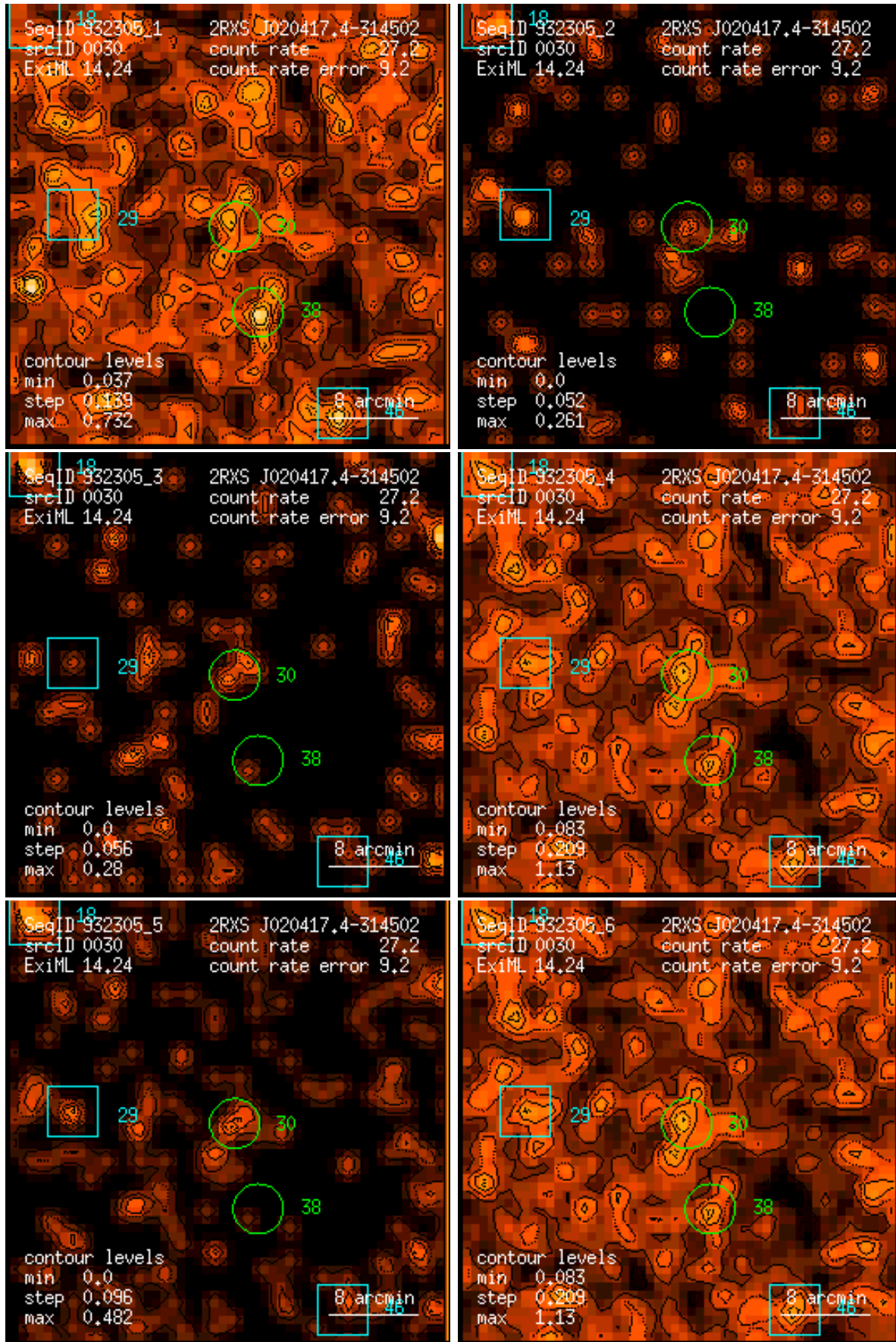
Figure 30: RASS 932305: detection 0030: band rate images, Gaussian filter: (1) PSPC channels 11 – 41, (2) 52 – 90, (3) 91 – 201, (4) 11 – 235, (5) 52 – 201, (6) 11 – 201. Broad band rates in counts/ks. Band rate contour levels in counts/ks/arcmin 2 .
