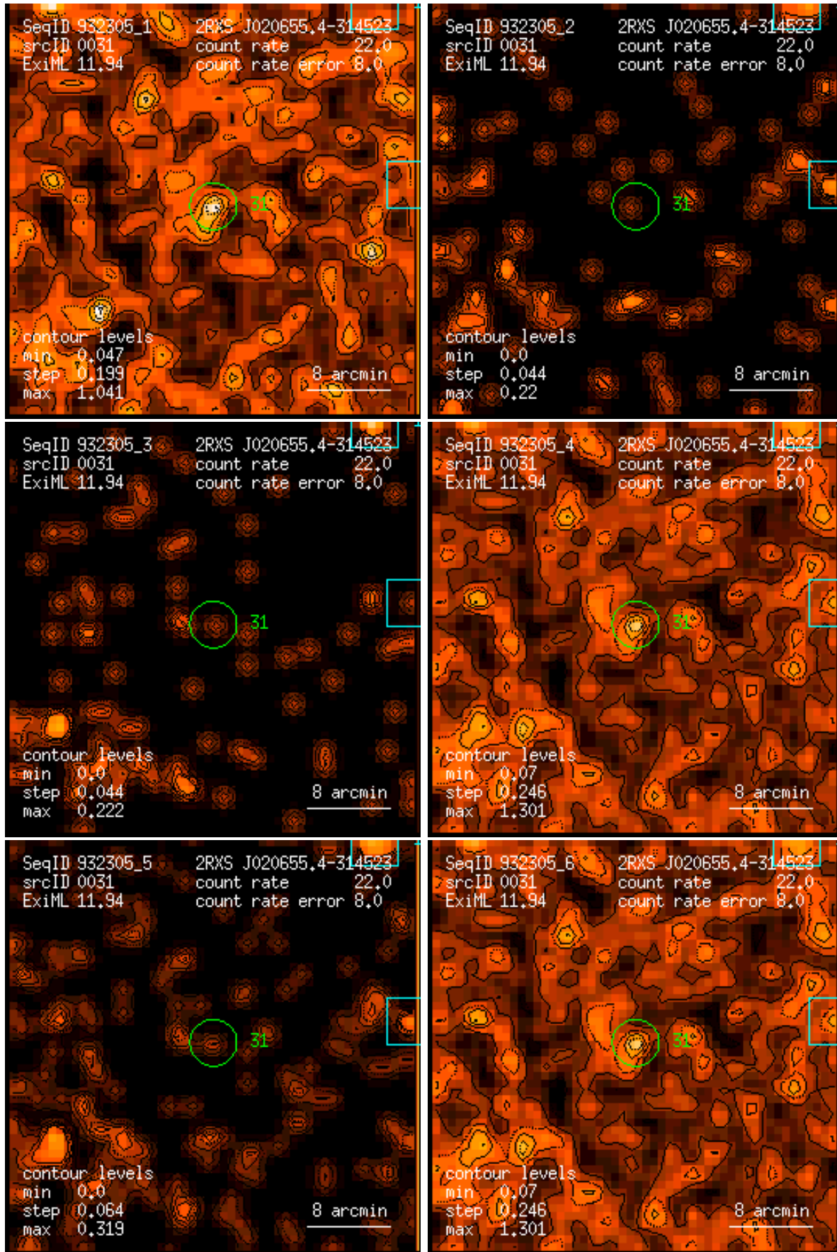
Figure 31: RASS 932305: detection 0031: band rate images, Gaussian filter: (1) PSPC channels 11 – 41, (2) 52 – 90, (3) 91 – 201, (4) 11 – 235, (5) 52 – 201, (6) 11 – 201. Broad band rates in counts/ks. Band rate contour levels in counts/ks/arcmin 2 .
