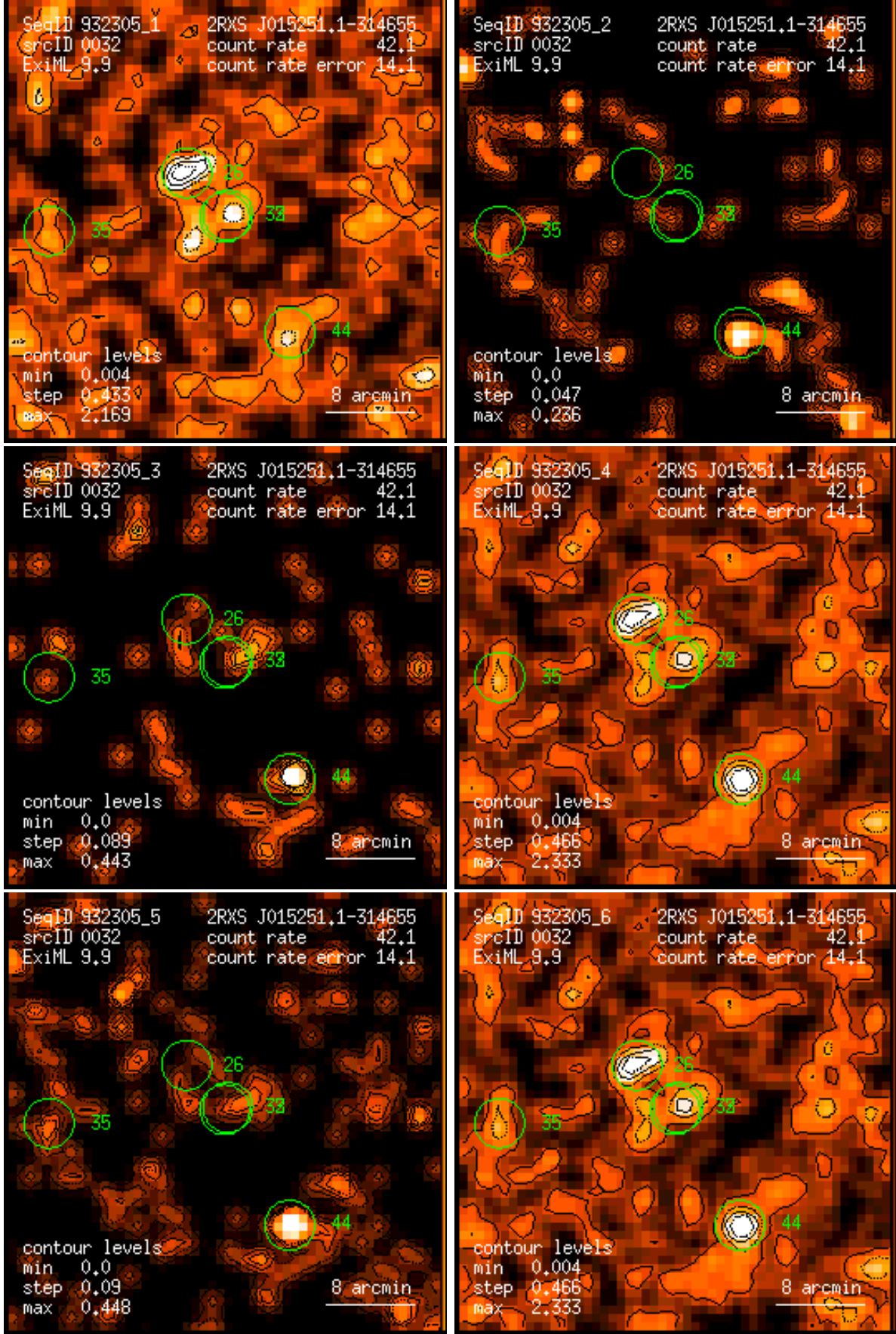
Figure 32: RASS 932305: detection 0032: band rate images, Gaussian filter: (1) PSPC channels 11 – 41, (2) 52 – 90, (3) 91 – 201, (4) 11 – 235, (5) 52 – 201, (6) 11 – 201. Broad band rates in counts/ks. Band rate contour levels in counts/ks/arcmin 2 .
