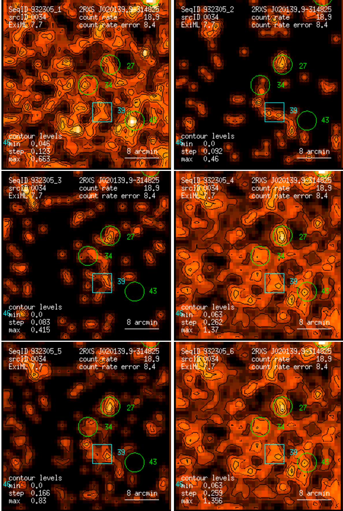
Figure 34: RASS 932305: detection 0034: band rate images, Gaussian filter: (1) PSPC channels 11 – 41, (2) 52 – 90, (3) 91 – 201, (4) 11 – 235, (5) 52 – 201, (6) 11 – 201. Broad band rates in counts/ks. Band rate contour levels in counts/ks/arcmin 2 .
