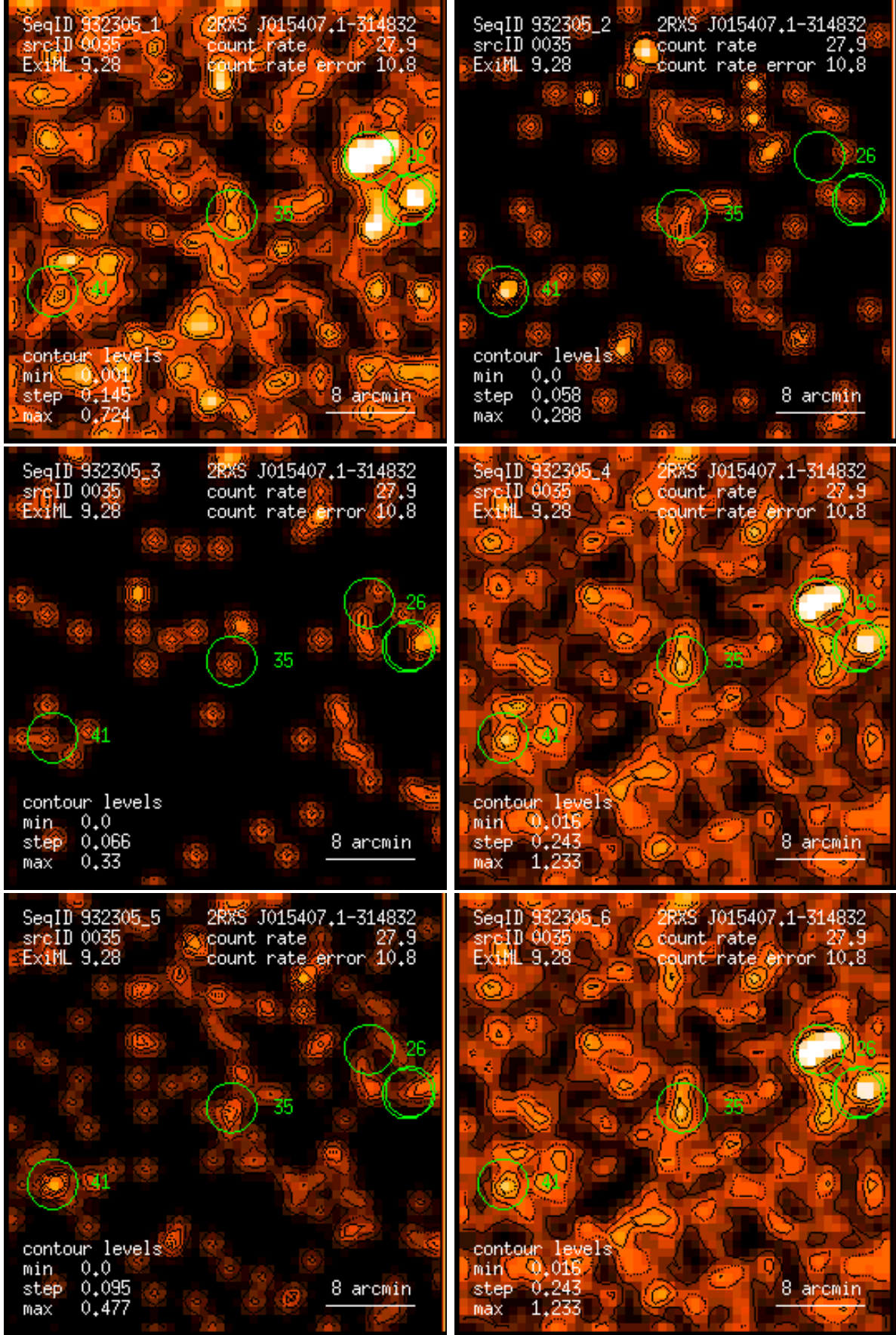
Figure 35: RASS 932305: detection 0035: band rate images, Gaussian filter: (1) PSPC channels 11 – 41, (2) 52 – 90, (3) 91 – 201, (4) 11 – 235, (5) 52 – 201, (6) 11 – 201. Broad band rates in counts/ks. Band rate contour levels in counts/ks/arcmin 2 .
