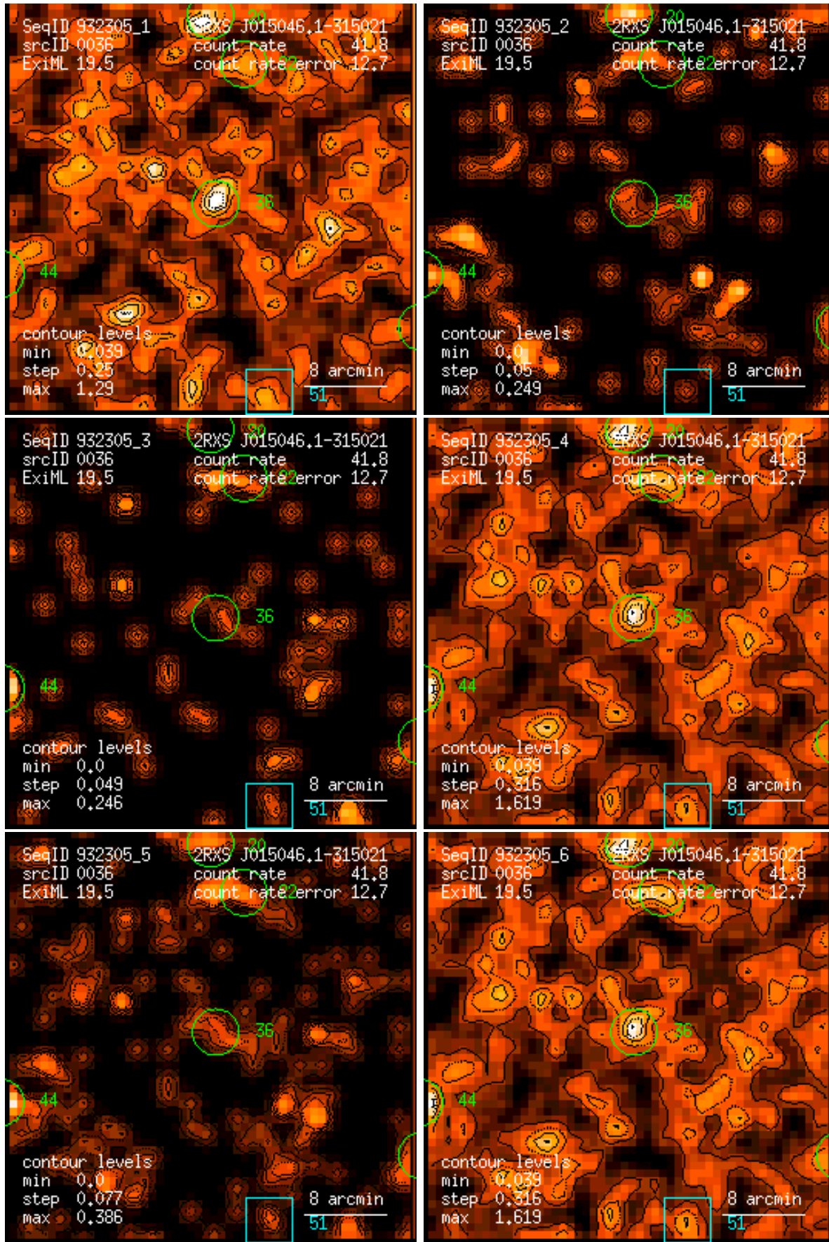
Figure 36: RASS 932305: detection 0036: band rate images, Gaussian filter: (1) PSPC channels 11 – 41, (2) 52 – 90, (3) 91 – 201, (4) 11 – 235, (5) 52 – 201, (6) 11 – 201. Broad band rates in counts/ks. Band rate contour levels in counts/ks/arcmin 2 .
