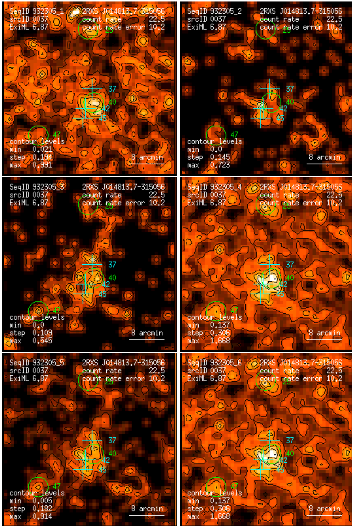
Figure 37: RASS 932305: detection 0037: band rate images, Gaussian filter: (1) PSPC channels 11 – 41, (2) 52 – 90, (3) 91 – 201, (4) 11 – 235, (5) 52 – 201, (6) 11 – 201. Broad band rates in counts/ks. Band rate contour levels in counts/ks/arcmin 2 .
