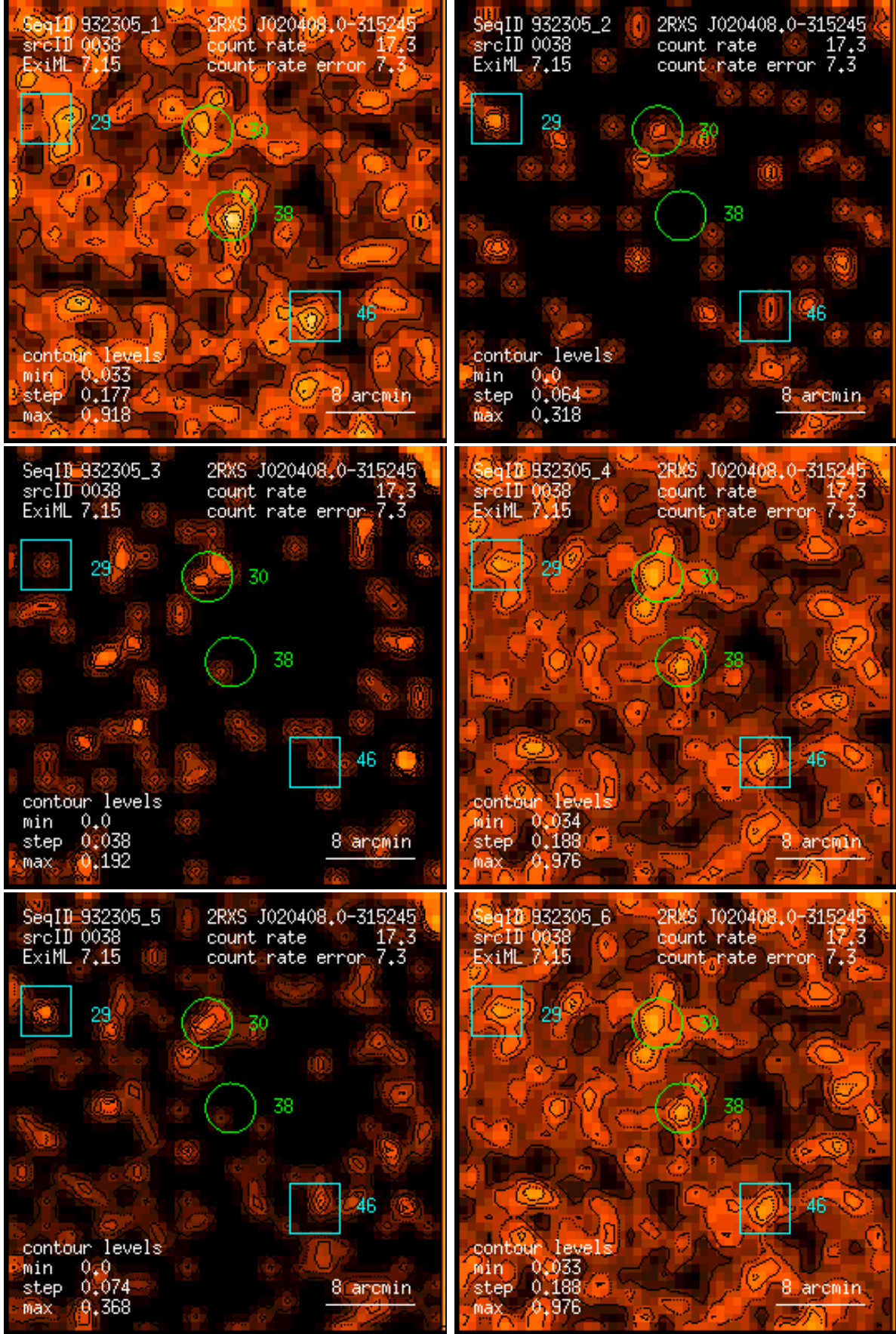
Figure 38: RASS 932305: detection 0038: band rate images, Gaussian filter: (1) PSPC channels 11 – 41, (2) 52 – 90, (3) 91 – 201, (4) 11 – 235, (5) 52 – 201, (6) 11 – 201. Broad band rates in counts/ks. Band rate contour levels in counts/ks/arcmin 2 .
