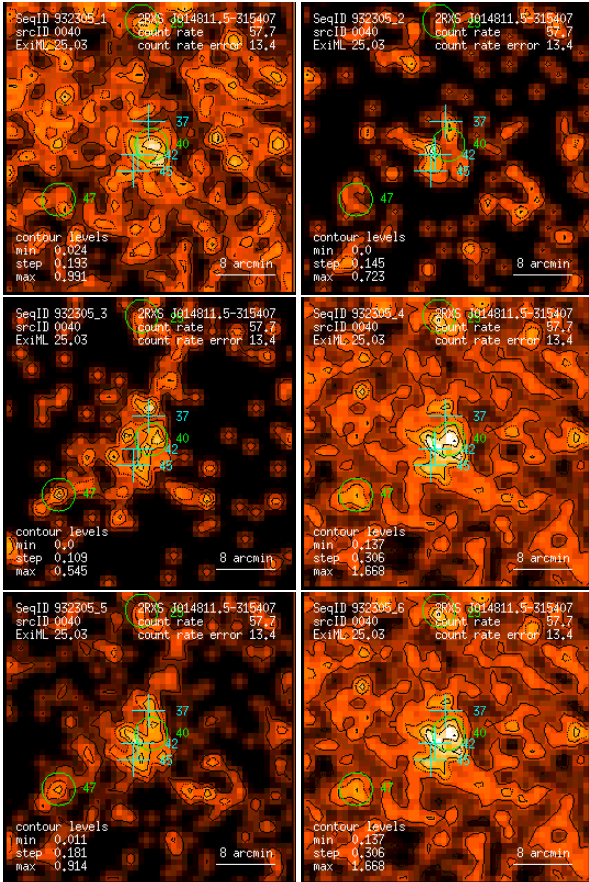
Figure 40: RASS 932305: detection 0040: band rate images, Gaussian filter: (1) PSPC channels 11 – 41, (2) 52 – 90, (3) 91 – 201, (4) 11 – 235, (5) 52 – 201, (6) 11 – 201. Broad band rates in counts/ks. Band rate contour levels in counts/ks/arcmin 2 .
