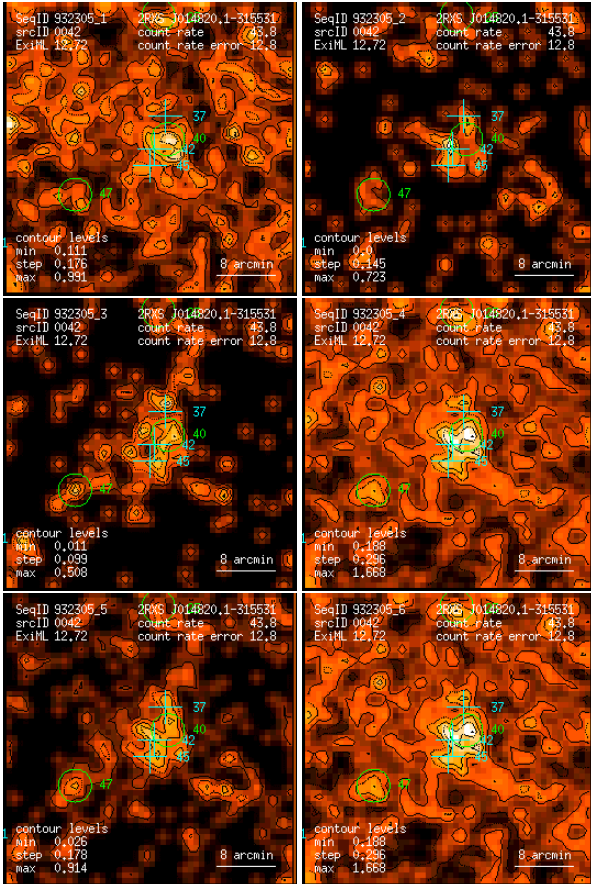
Figure 42: RASS 932305: detection 0042: band rate images, Gaussian filter: (1) PSPC channels 11 – 41, (2) 52 – 90, (3) 91 – 201, (4) 11 – 235, (5) 52 – 201, (6) 11 – 201. Broad band rates in counts/ks. Band rate contour levels in counts/ks/arcmin 2 .
