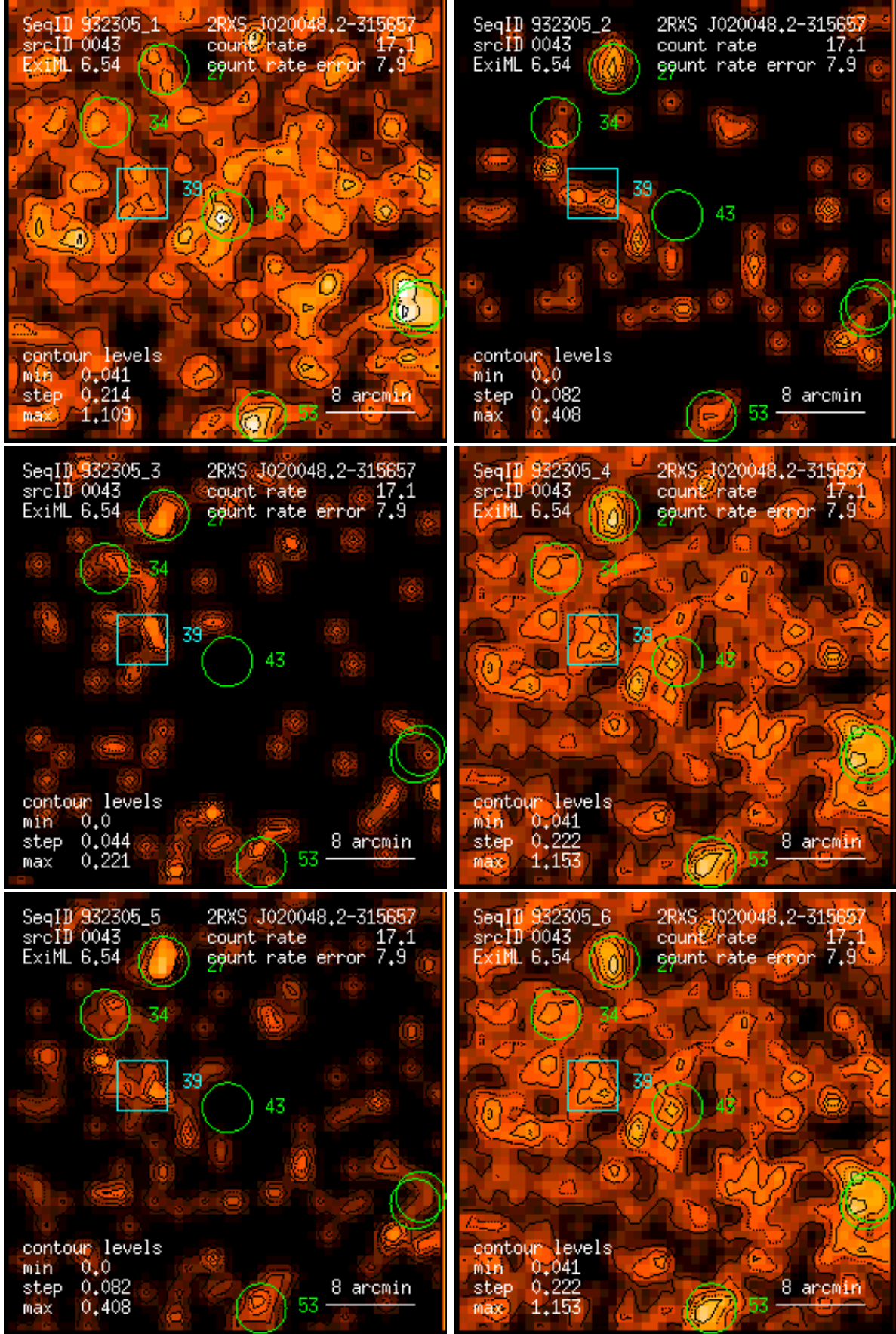
Figure 43: RASS 932305: detection 0043: band rate images, Gaussian filter: (1) PSPC channels 11 – 41, (2) 52 – 90, (3) 91 – 201, (4) 11 – 235, (5) 52 – 201, (6) 11 – 201. Broad band rates in counts/ks. Band rate contour levels in counts/ks/arcmin 2 .
