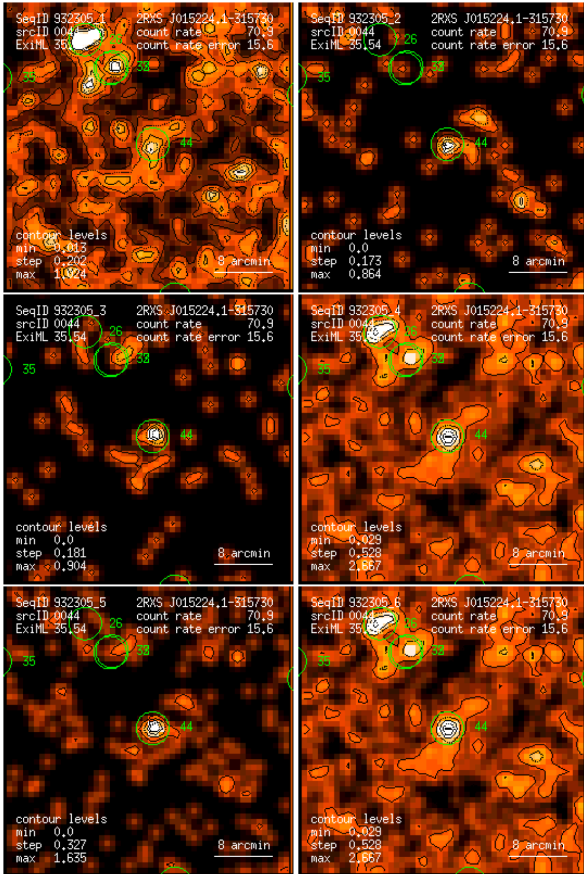
Figure 44: RASS 932305: detection 0044: band rate images, Gaussian filter: (1) PSPC channels 11 – 41, (2) 52 – 90, (3) 91 – 201, (4) 11 – 235, (5) 52 – 201, (6) 11 – 201. Broad band rates in counts/ks. Band rate contour levels in counts/ks/arcmin 2 .
