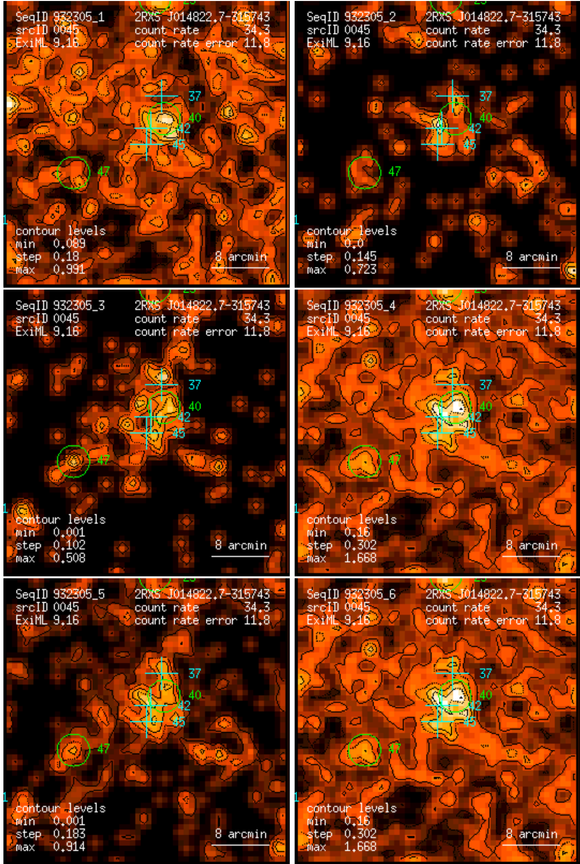
Figure 45: RASS 932305: detection 0045: band rate images, Gaussian filter: (1) PSPC channels 11 – 41, (2) 52 – 90, (3) 91 – 201, (4) 11 – 235, (5) 52 – 201, (6) 11 – 201. Broad band rates in counts/ks. Band rate contour levels in counts/ks/arcmin 2 .
