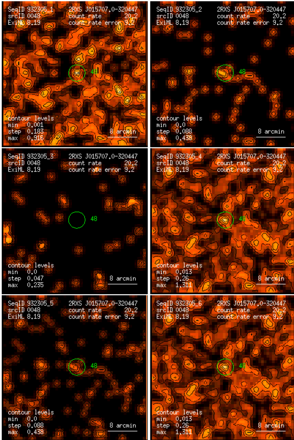
Figure 48: RASS 932305: detection 0048: band rate images, Gaussian filter: (1) PSPC channels 11 – 41, (2) 52 – 90, (3) 91 – 201, (4) 11 – 235, (5) 52 – 201, (6) 11 – 201. Broad band rates in counts/ks. Band rate contour levels in counts/ks/arcmin 2 .
