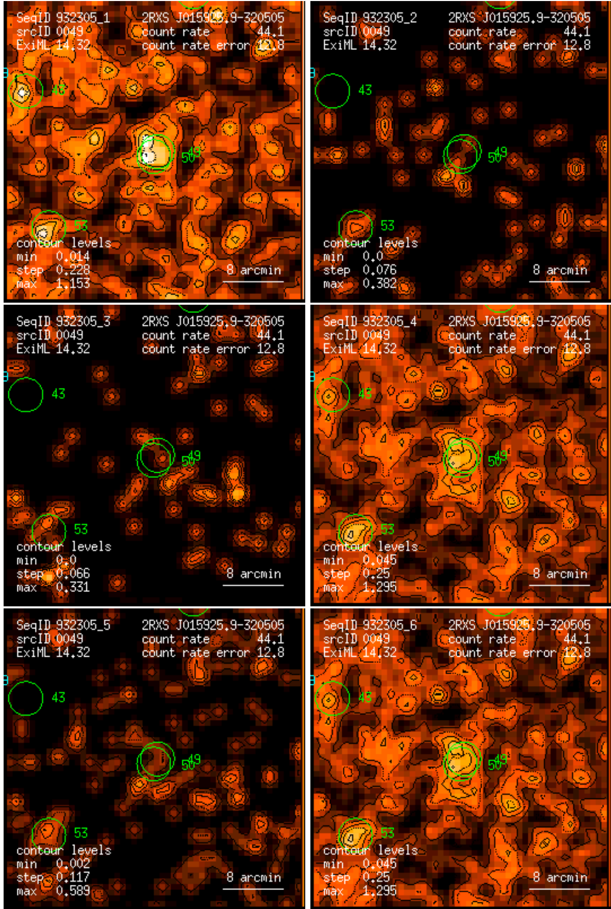
Figure 49: RASS 932305: detection 0049: band rate images, Gaussian filter: (1) PSPC channels 11 – 41, (2) 52 – 90, (3) 91 – 201, (4) 11 – 235, (5) 52 – 201, (6) 11 – 201. Broad band rates in counts/ks. Band rate contour levels in counts/ks/arcmin 2 .
