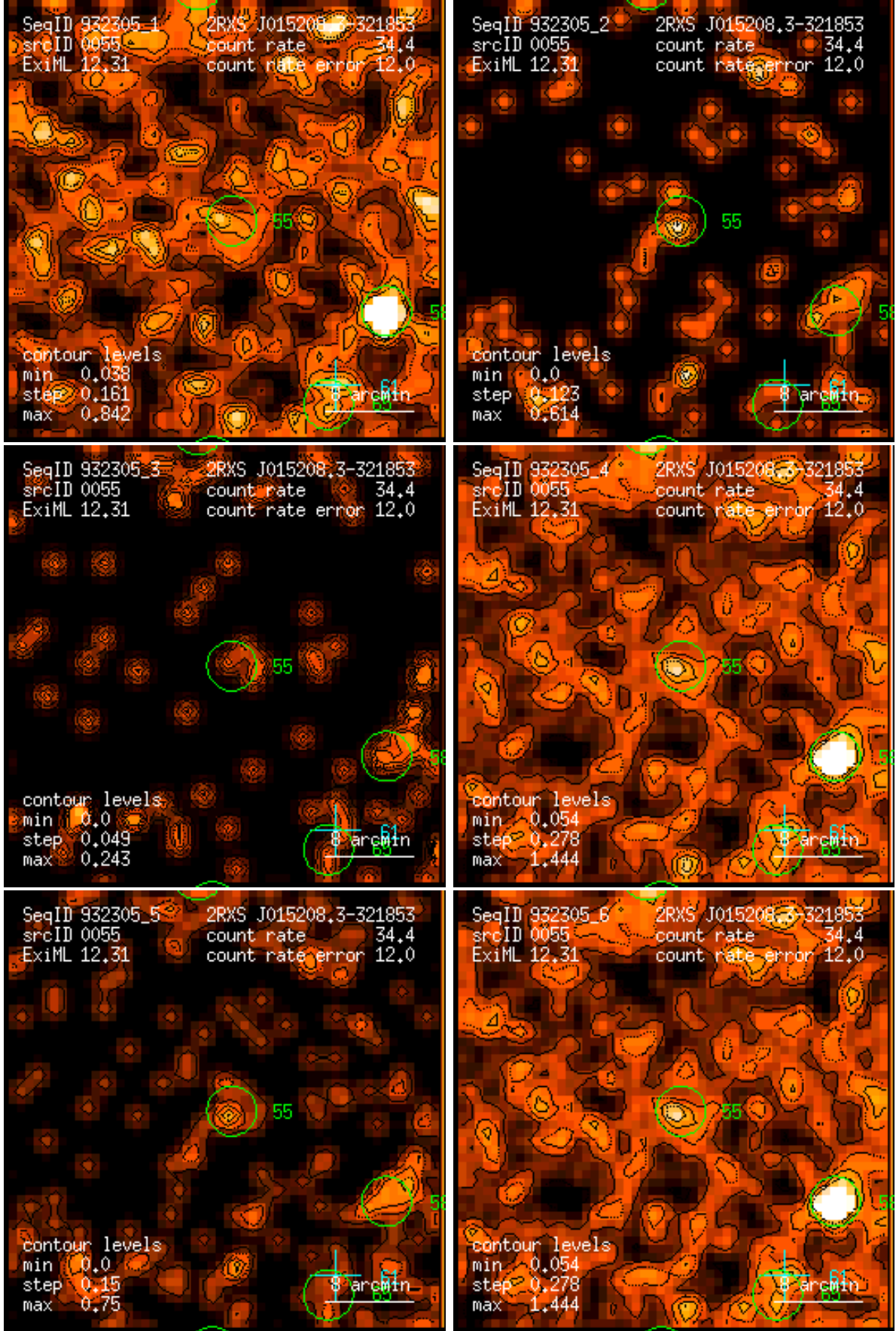
Figure 55: RASS 932305: detection 0055: band rate images, Gaussian filter: (1) PSPC channels 11 – 41, (2) 52 – 90, (3) 91 – 201, (4) 11 – 235, (5) 52 – 201, (6) 11 – 201. Broad band rates in counts/ks. Band rate contour levels in counts/ks/arcmin 2 .
