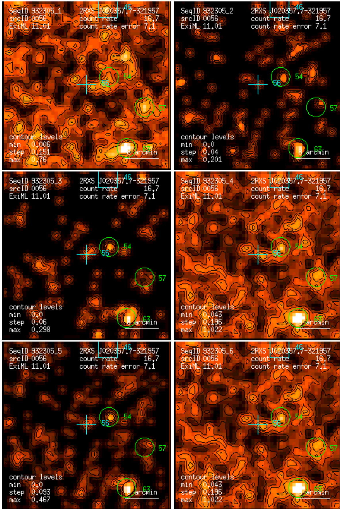
Figure 56: RASS 932305: detection 0056: band rate images, Gaussian filter: (1) PSPC channels 11 – 41, (2) 52 – 90, (3) 91 – 201, (4) 11 – 235, (5) 52 – 201, (6) 11 – 201. Broad band rates in counts/ks. Band rate contour levels in counts/ks/arcmin 2 .
