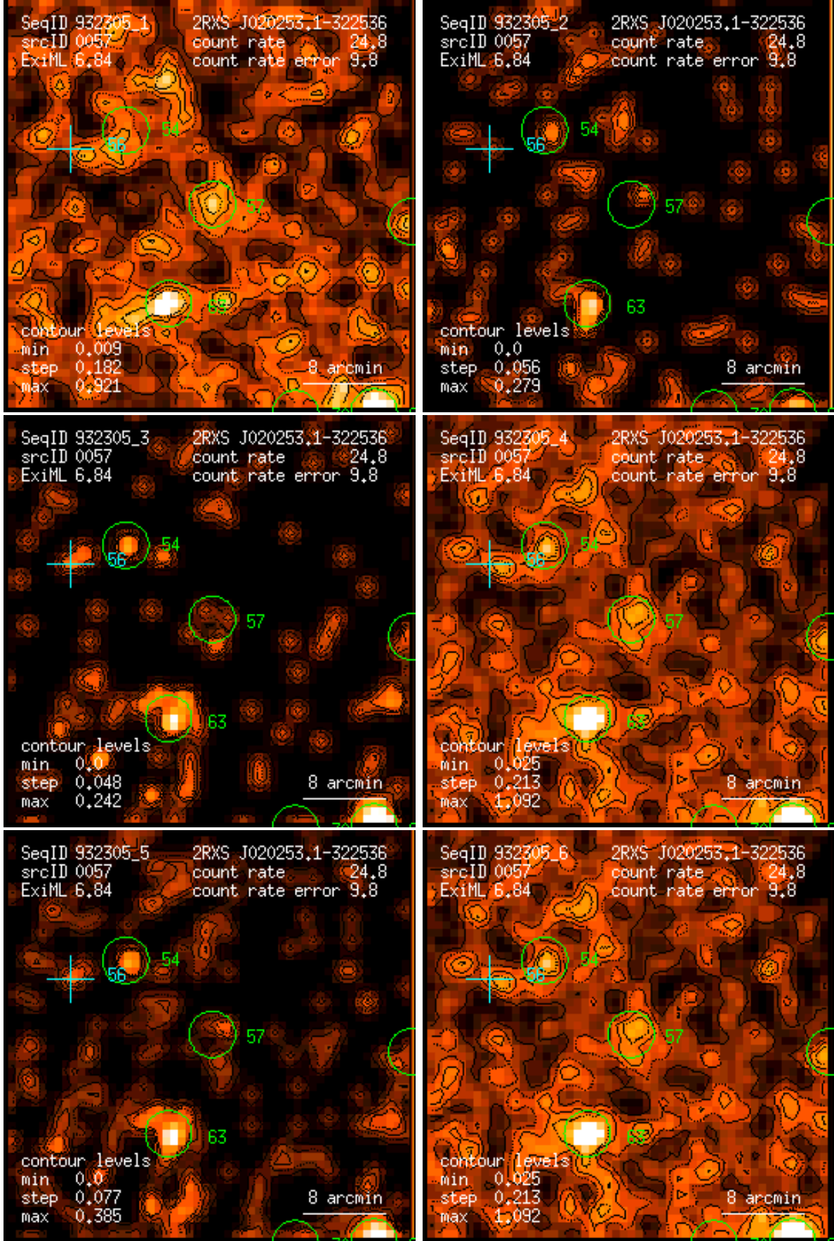
Figure 57: RASS 932305: detection 0057: band rate images, Gaussian filter: (1) PSPC channels 11 – 41, (2) 52 – 90, (3) 91 – 201, (4) 11 – 235, (5) 52 – 201, (6) 11 – 201. Broad band rates in counts/ks. Band rate contour levels in counts/ks/arcmin 2 .
