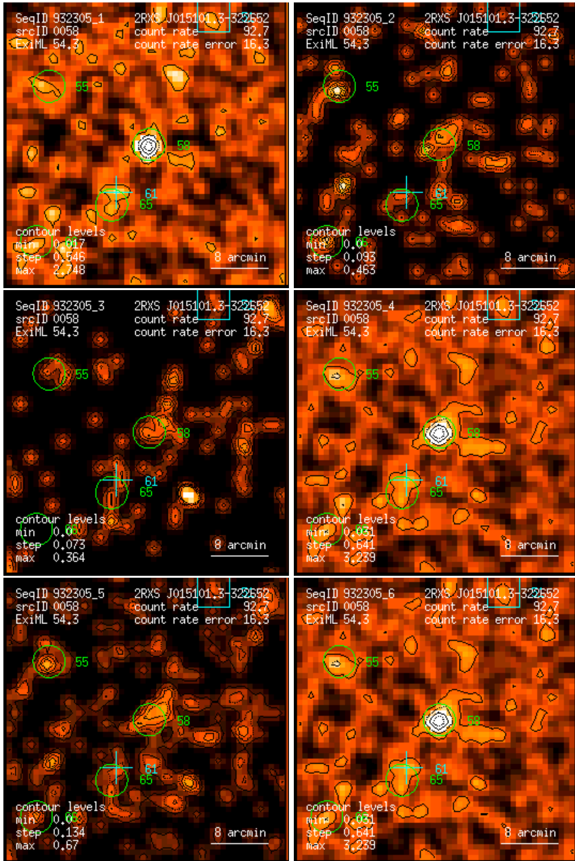
Figure 58: RASS 932305: detection 0058: band rate images, Gaussian filter: (1) PSPC channels 11 – 41, (2) 52 – 90, (3) 91 – 201, (4) 11 – 235, (5) 52 – 201, (6) 11 – 201. Broad band rates in counts/ks. Band rate contour levels in counts/ks/arcmin 2 .
