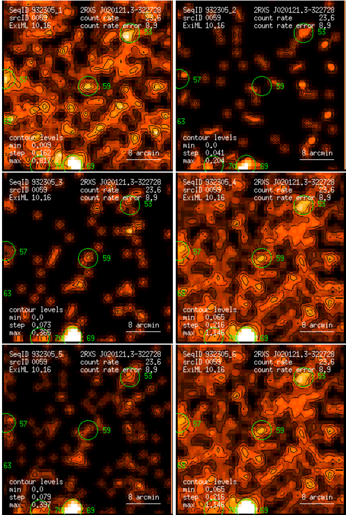
Figure 59: RASS 932305: detection 0059: band rate images, Gaussian filter: (1) PSPC channels 11 – 41, (2) 52 – 90, (3) 91 – 201, (4) 11 – 235, (5) 52 – 201, (6) 11 – 201. Broad band rates in counts/ks. Band rate contour levels in counts/ks/arcmin 2 .
