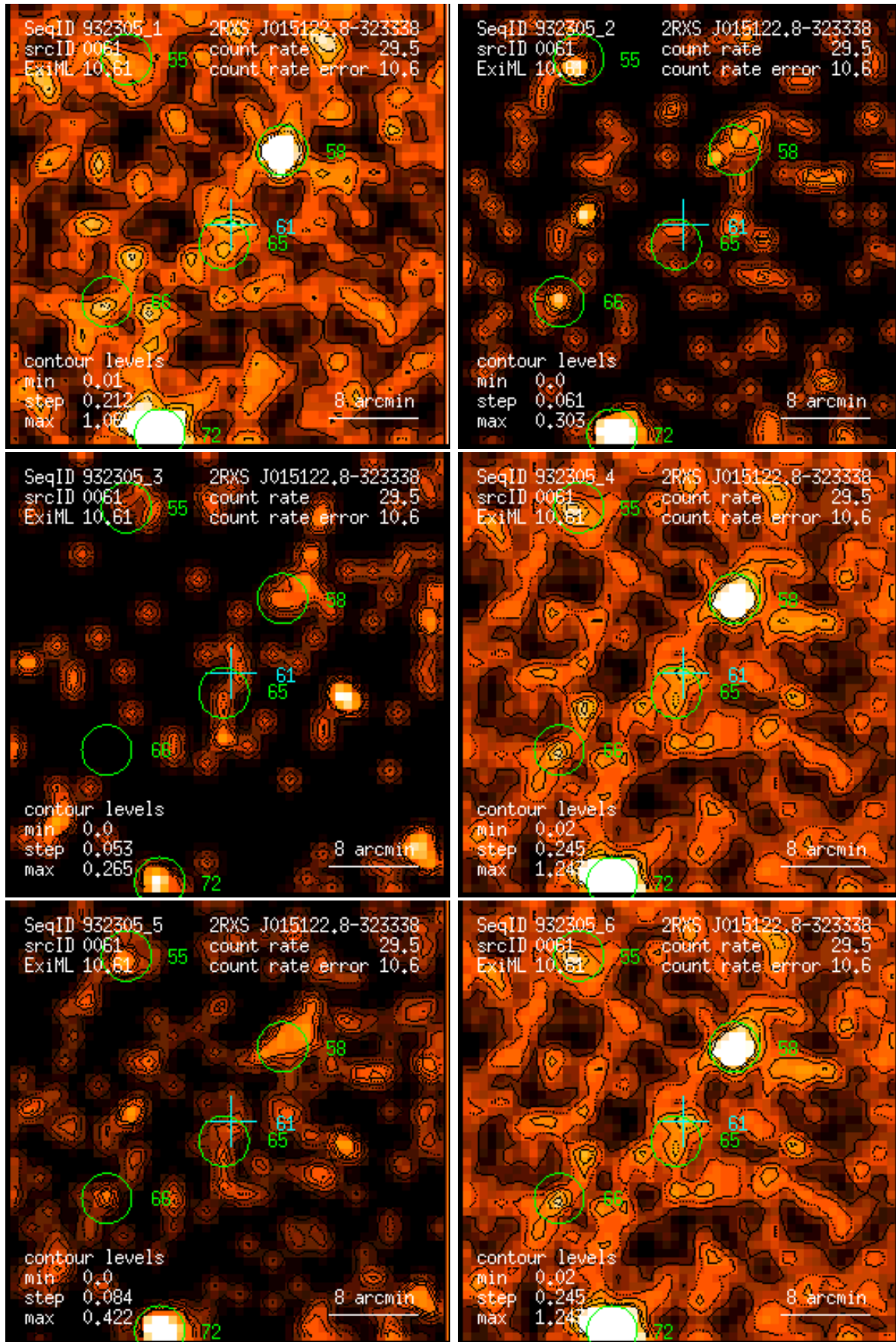
Figure 61: RASS 932305: detection 0061: band rate images, Gaussian filter: (1) PSPC channels 11 – 41, (2) 52 – 90, (3) 91 – 201, (4) 11 – 235, (5) 52 – 201, (6) 11 – 201. Broad band rates in counts/ks. Band rate contour levels in counts/ks/arcmin 2 .
