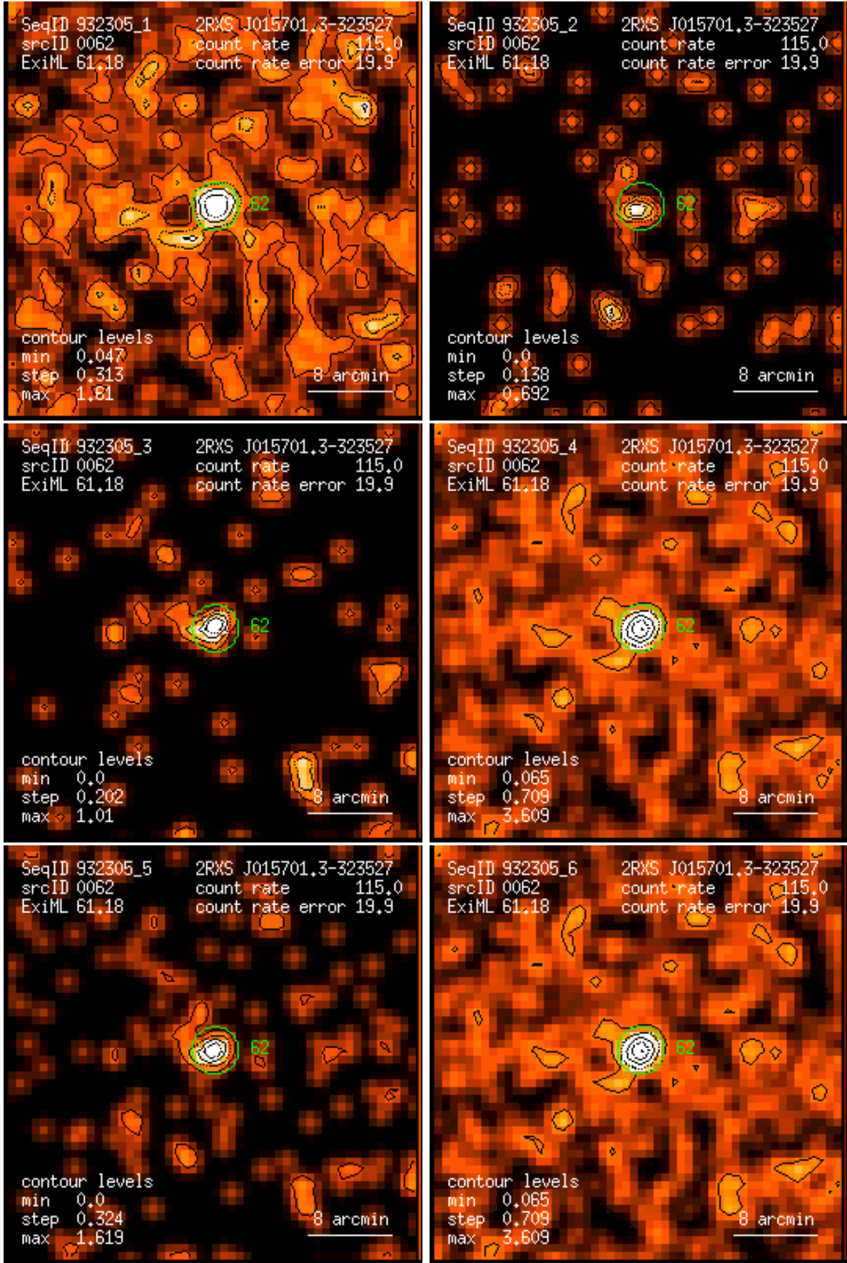
Figure 62: RASS 932305: detection 0062: band rate images, Gaussian filter: (1) PSPC channels 11 – 41, (2) 52 – 90, (3) 91 – 201, (4) 11 – 235, (5) 52 – 201, (6) 11 – 201. Broad band rates in counts/ks. Band rate contour levels in counts/ks/arcmin 2 .
