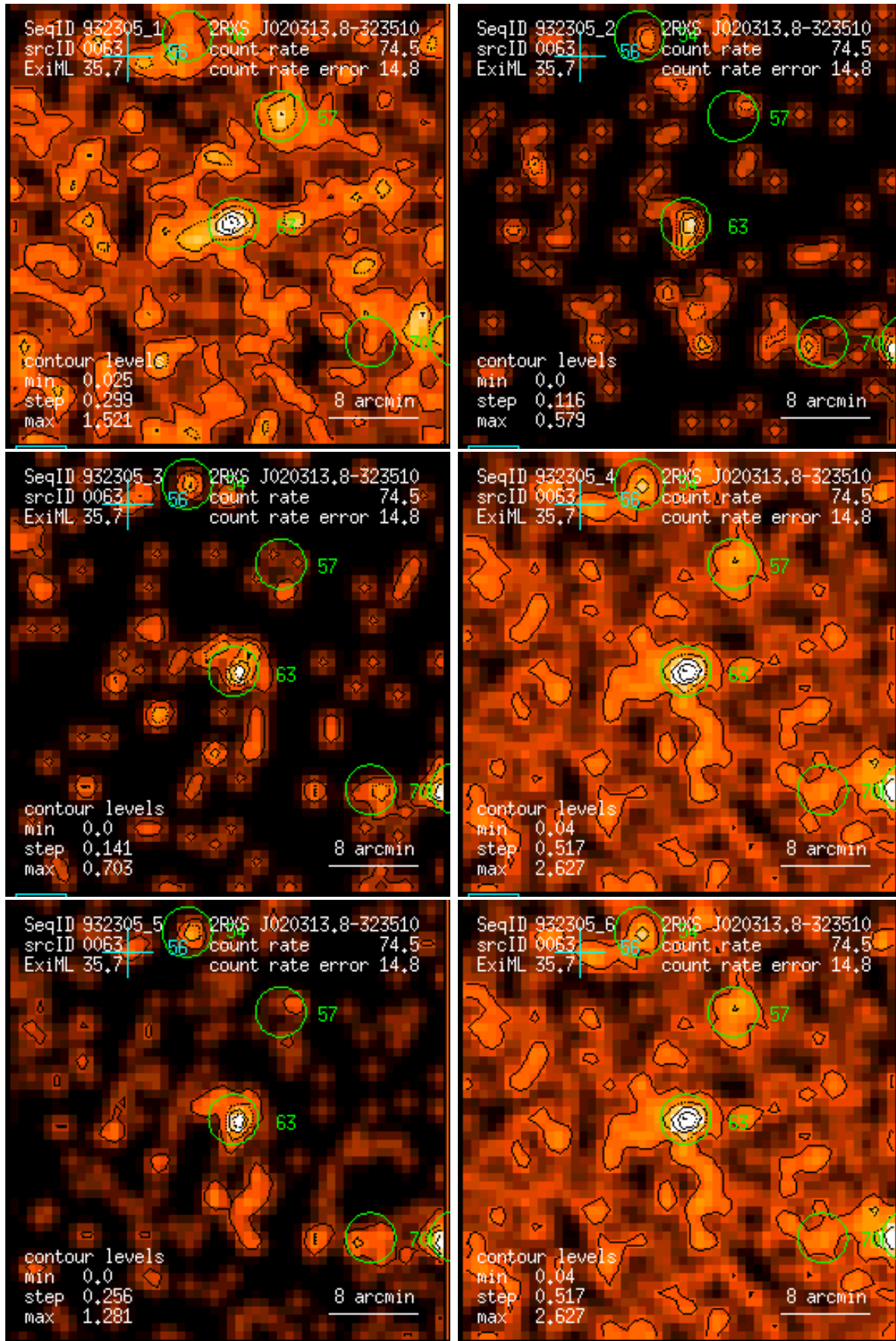
Figure 63: RASS 932305: detection 0063: band rate images, Gaussian filter: (1) PSPC channels 11 – 41, (2) 52 – 90, (3) 91 – 201, (4) 11 – 235, (5) 52 – 201, (6) 11 – 201. Broad band rates in counts/ks. Band rate contour levels in counts/ks/arcmin 2 .
