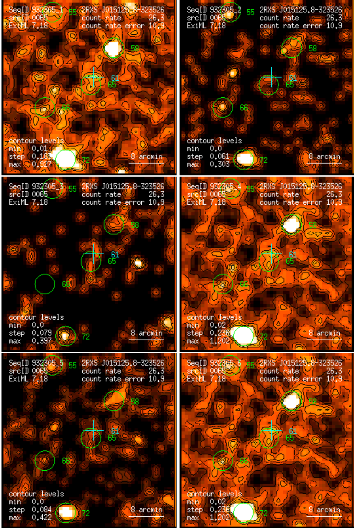
Figure 65: RASS 932305: detection 0065: band rate images, Gaussian filter: (1) PSPC channels 11 – 41, (2) 52 – 90, (3) 91 – 201, (4) 11 – 235, (5) 52 – 201, (6) 11 – 201. Broad band rates in counts/ks. Band rate contour levels in counts/ks/arcmin 2 .
