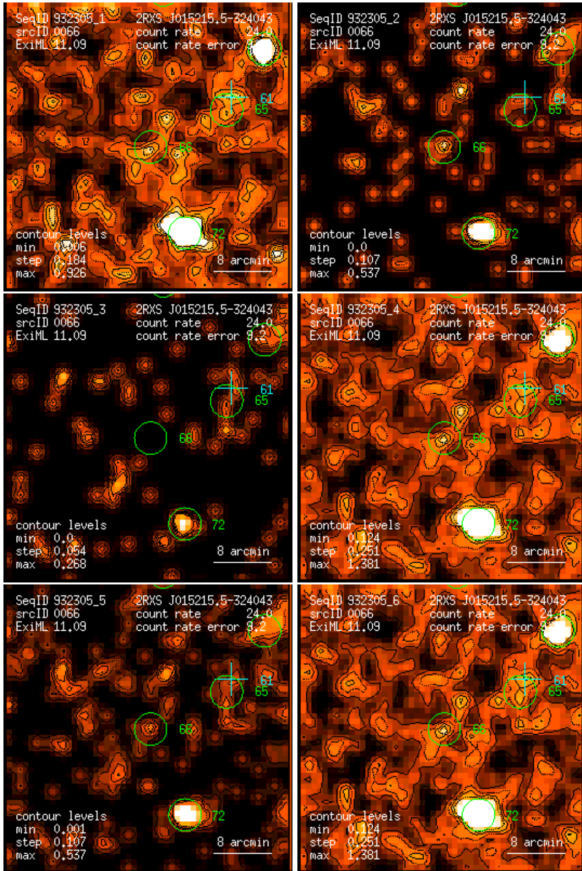
Figure 66: RASS 932305: detection 0066: band rate images, Gaussian filter: (1) PSPC channels 11 – 41, (2) 52 – 90, (3) 91 – 201, (4) 11 – 235, (5) 52 – 201, (6) 11 – 201. Broad band rates in counts/ks. Band rate contour levels in counts/ks/arcmin 2 .
