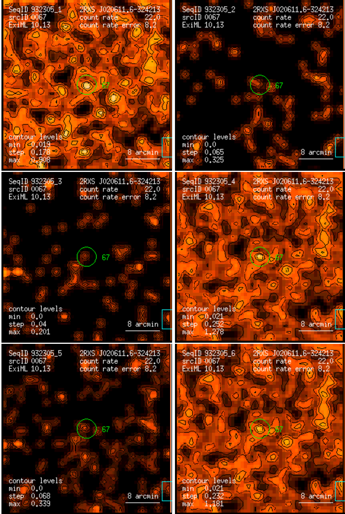
Figure 67: RASS 932305: detection 0067: band rate images, Gaussian filter: (1) PSPC channels 11 – 41, (2) 52 – 90, (3) 91 – 201, (4) 11 – 235, (5) 52 – 201, (6) 11 – 201. Broad band rates in counts/ks. Band rate contour levels in counts/ks/arcmin 2 .
