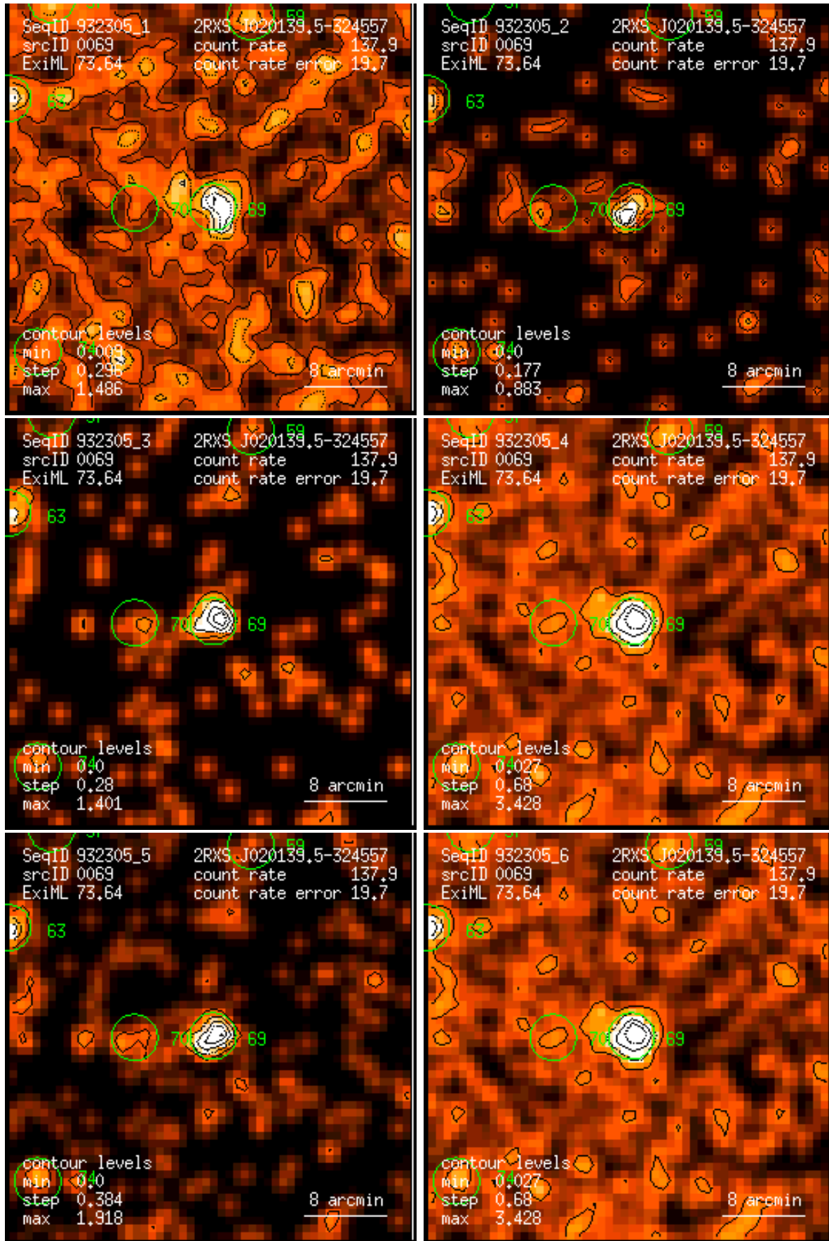
Figure 69: RASS 932305: detection 0069: band rate images, Gaussian filter: (1) PSPC channels 11 – 41, (2) 52 – 90, (3) 91 – 201, (4) 11 – 235, (5) 52 – 201, (6) 11 – 201. Broad band rates in counts/ks. Band rate contour levels in counts/ks/arcmin 2 .
