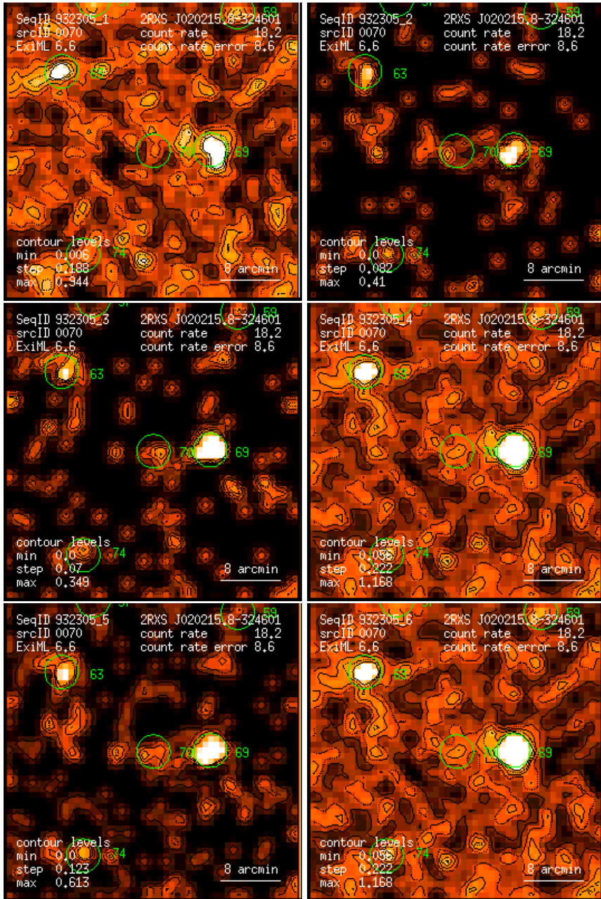
Figure 70: RASS 932305: detection 0070: band rate images, Gaussian filter: (1) PSPC channels 11 – 41, (2) 52 – 90, (3) 91 – 201, (4) 11 – 235, (5) 52 – 201, (6) 11 – 201. Broad band rates in counts/ks. Band rate contour levels in counts/ks/arcmin 2 .
