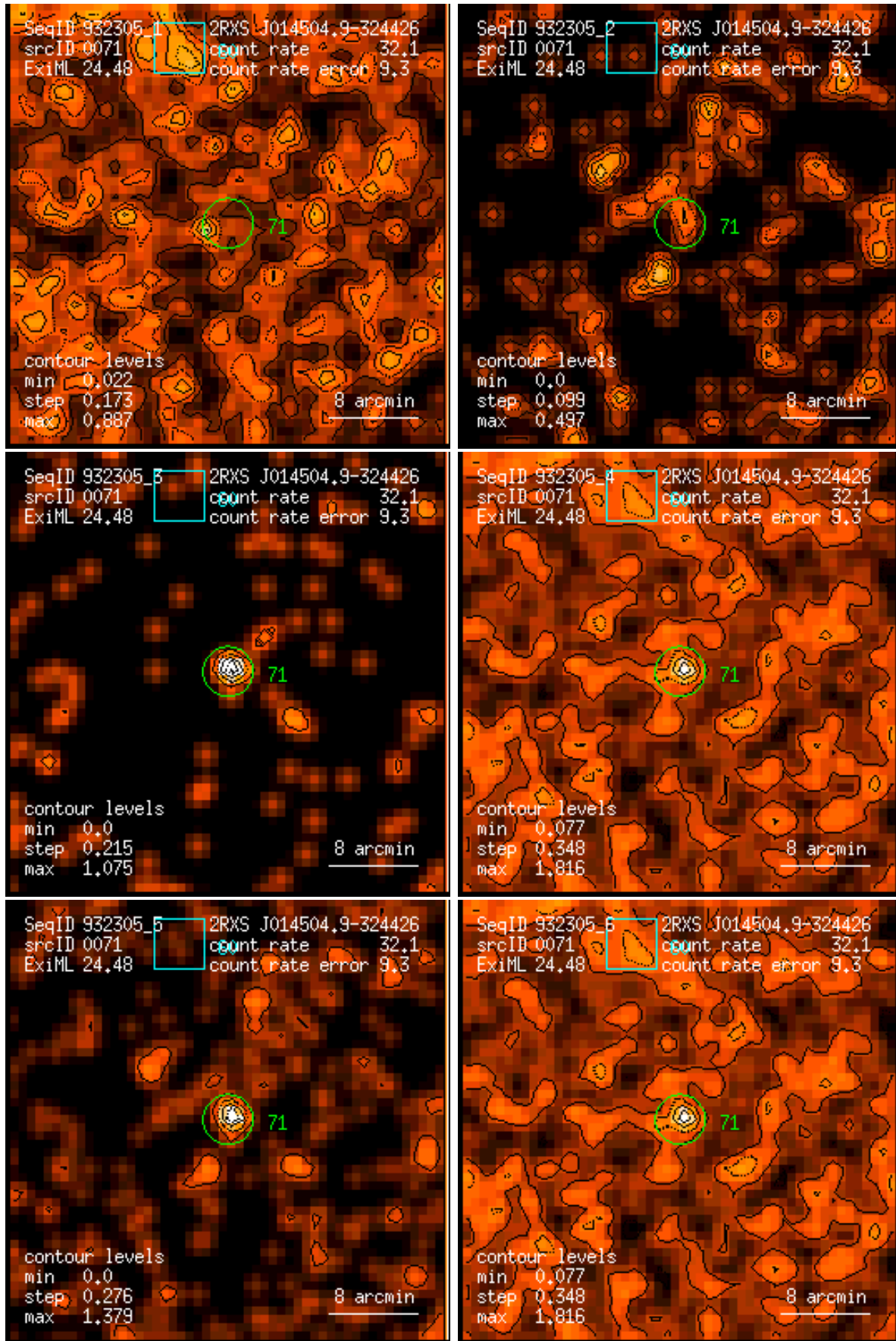
Figure 71: RASS 932305: detection 0071: band rate images, Gaussian filter: (1) PSPC channels 11 – 41, (2) 52 – 90, (3) 91 – 201, (4) 11 – 235, (5) 52 – 201, (6) 11 – 201. Broad band rates in counts/ks. Band rate contour levels in counts/ks/arcmin 2 .
