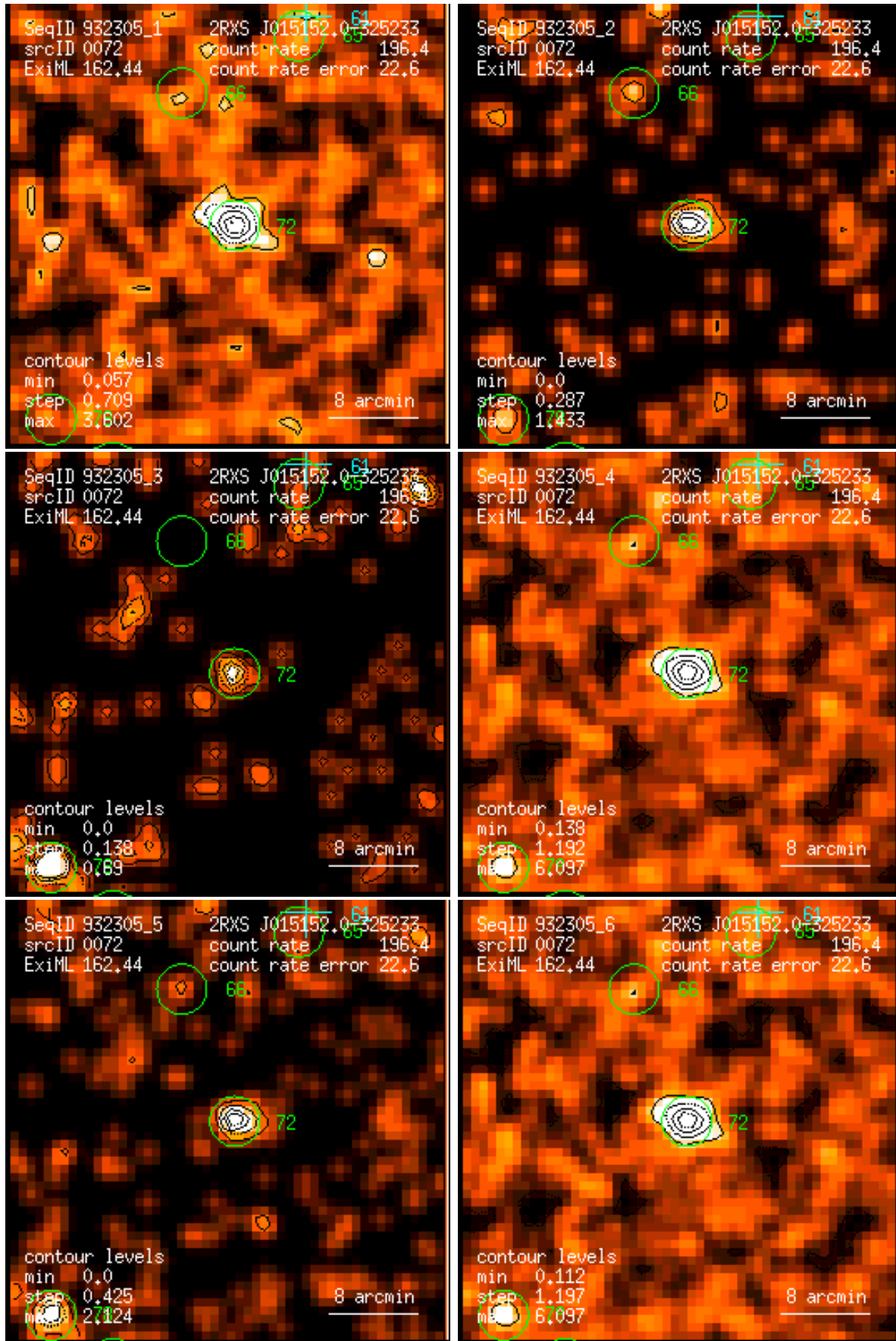
Figure 72: RASS 932305: detection 0072: band rate images, Gaussian filter: (1) PSPC channels 11 – 41, (2) 52 – 90, (3) 91 – 201, (4) 11 – 235, (5) 52 – 201, (6) 11 – 201. Broad band rates in counts/ks. Band rate contour levels in counts/ks/arcmin 2 .
