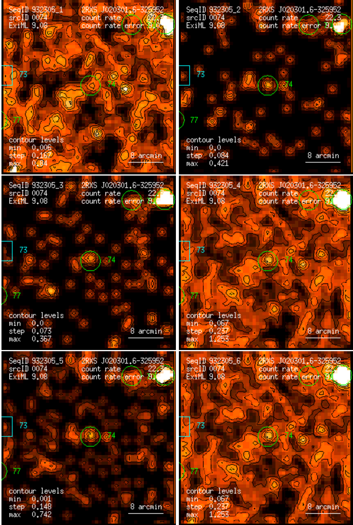
Figure 74: RASS 932305: detection 0074: band rate images, Gaussian filter: (1) PSPC channels 11 – 41, (2) 52 – 90, (3) 91 – 201, (4) 11 – 235, (5) 52 – 201, (6) 11 – 201. Broad band rates in counts/ks. Band rate contour levels in counts/ks/arcmin 2 .
