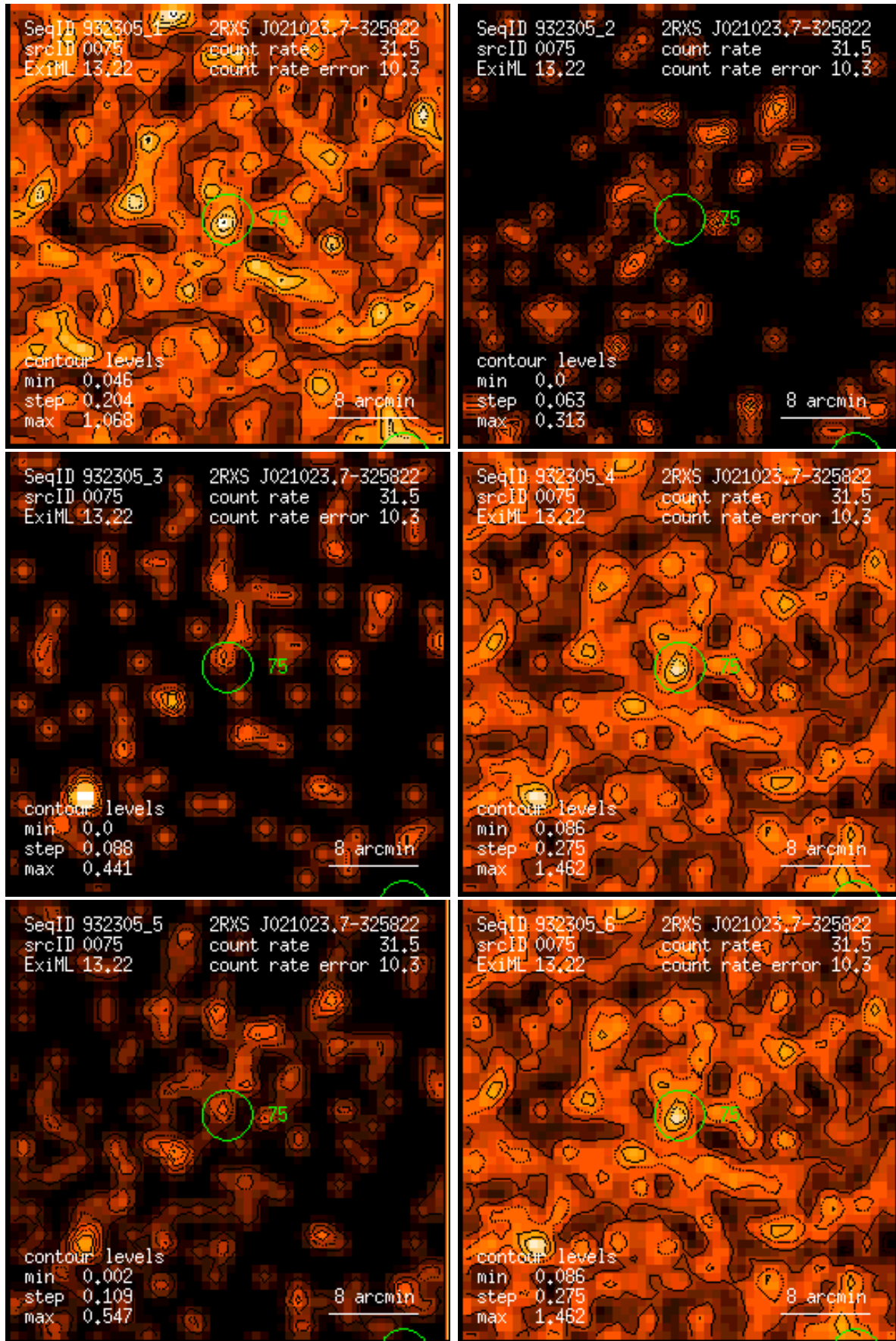
Figure 75: RASS 932305: detection 0075: band rate images, Gaussian filter: (1) PSPC channels 11 – 41, (2) 52 – 90, (3) 91 – 201, (4) 11 – 235, (5) 52 – 201, (6) 11 – 201. Broad band rates in counts/ks. Band rate contour levels in counts/ks/arcmin 2 .
