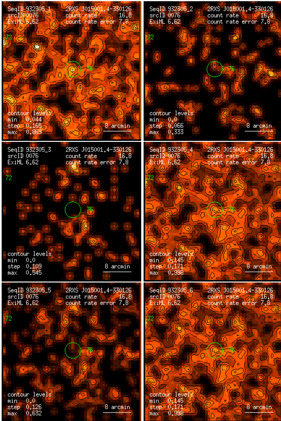
Figure 76: RASS 932305: detection 0076: band rate images, Gaussian filter: (1) PSPC channels 11 – 41, (2) 52 – 90, (3) 91 – 201, (4) 11 – 235, (5) 52 – 201, (6) 11 – 201. Broad band rates in counts/ks. Band rate contour levels in counts/ks/arcmin 2 .
