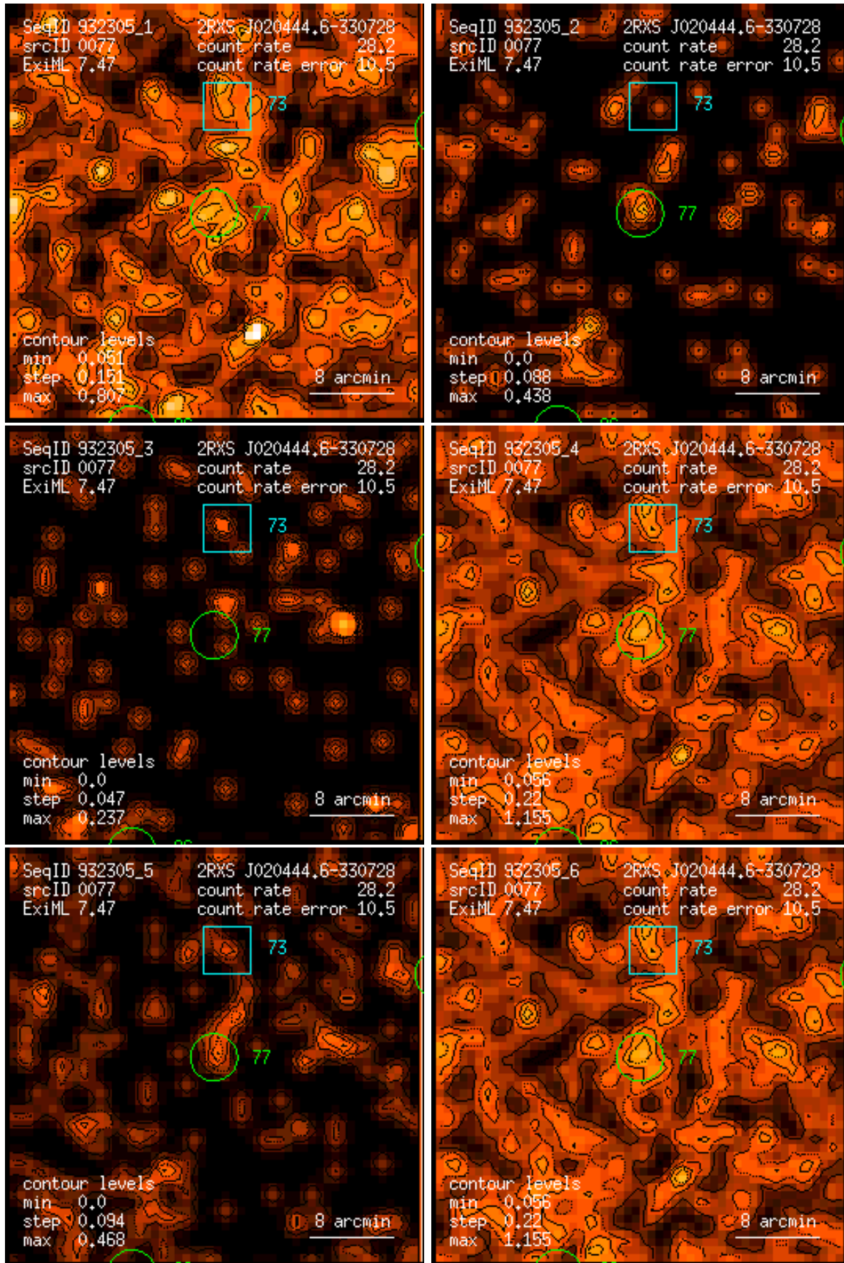
Figure 77: RASS 932305: detection 0077: band rate images, Gaussian filter: (1) PSPC channels 11 – 41, (2) 52 – 90, (3) 91 – 201, (4) 11 – 235, (5) 52 – 201, (6) 11 – 201. Broad band rates in counts/ks. Band rate contour levels in counts/ks/arcmin 2 .
