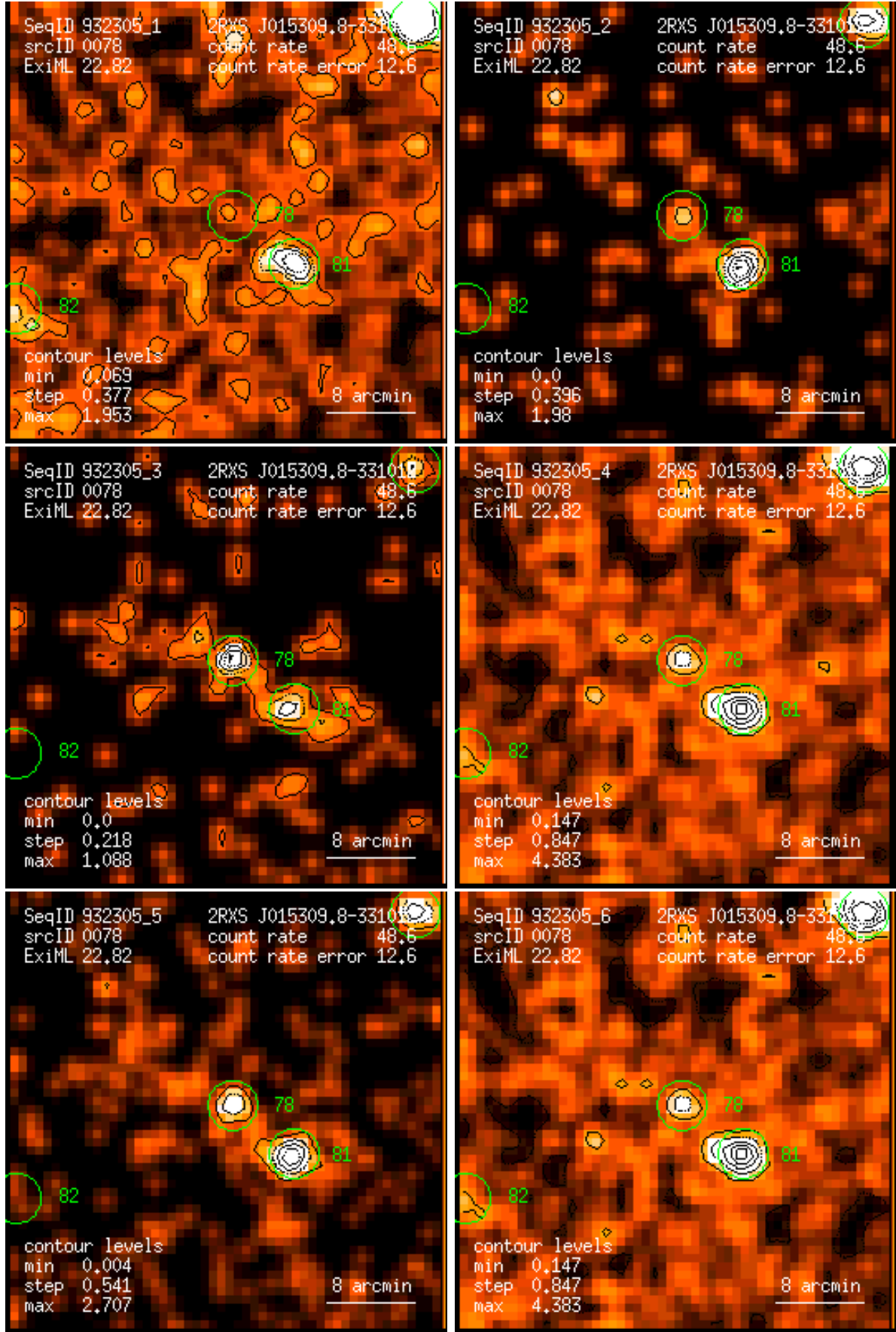
Figure 78: RASS 932305: detection 0078: band rate images, Gaussian filter: (1) PSPC channels 11 – 41, (2) 52 – 90, (3) 91 – 201, (4) 11 – 235, (5) 52 – 201, (6) 11 – 201. Broad band rates in counts/ks. Band rate contour levels in counts/ks/arcmin 2 .
