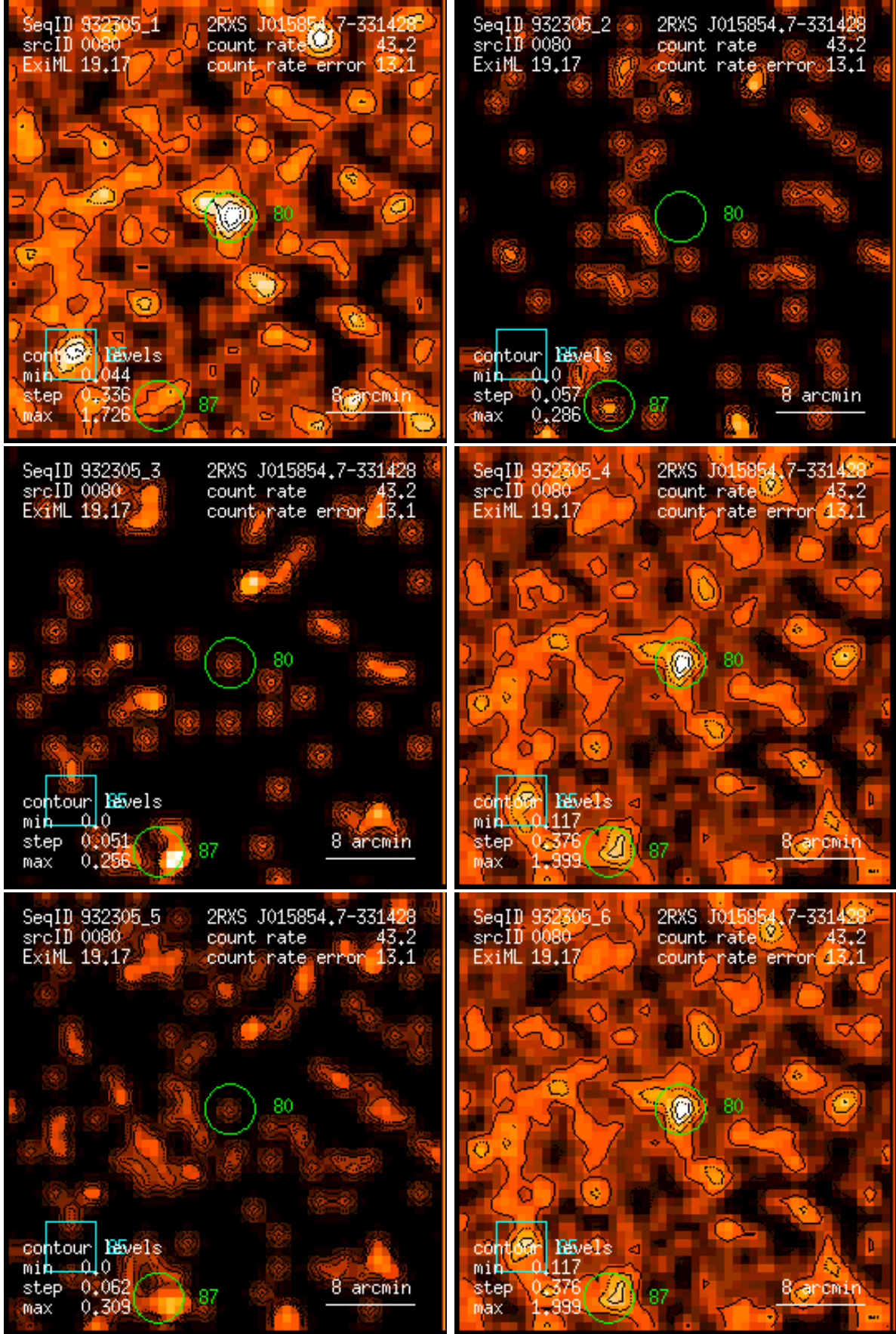
Figure 80: RASS 932305: detection 0080: band rate images, Gaussian filter: (1) PSPC channels 11 – 41, (2) 52 – 90, (3) 91 – 201, (4) 11 – 235, (5) 52 – 201, (6) 11 – 201. Broad band rates in counts/ks. Band rate contour levels in counts/ks/arcmin 2 .
