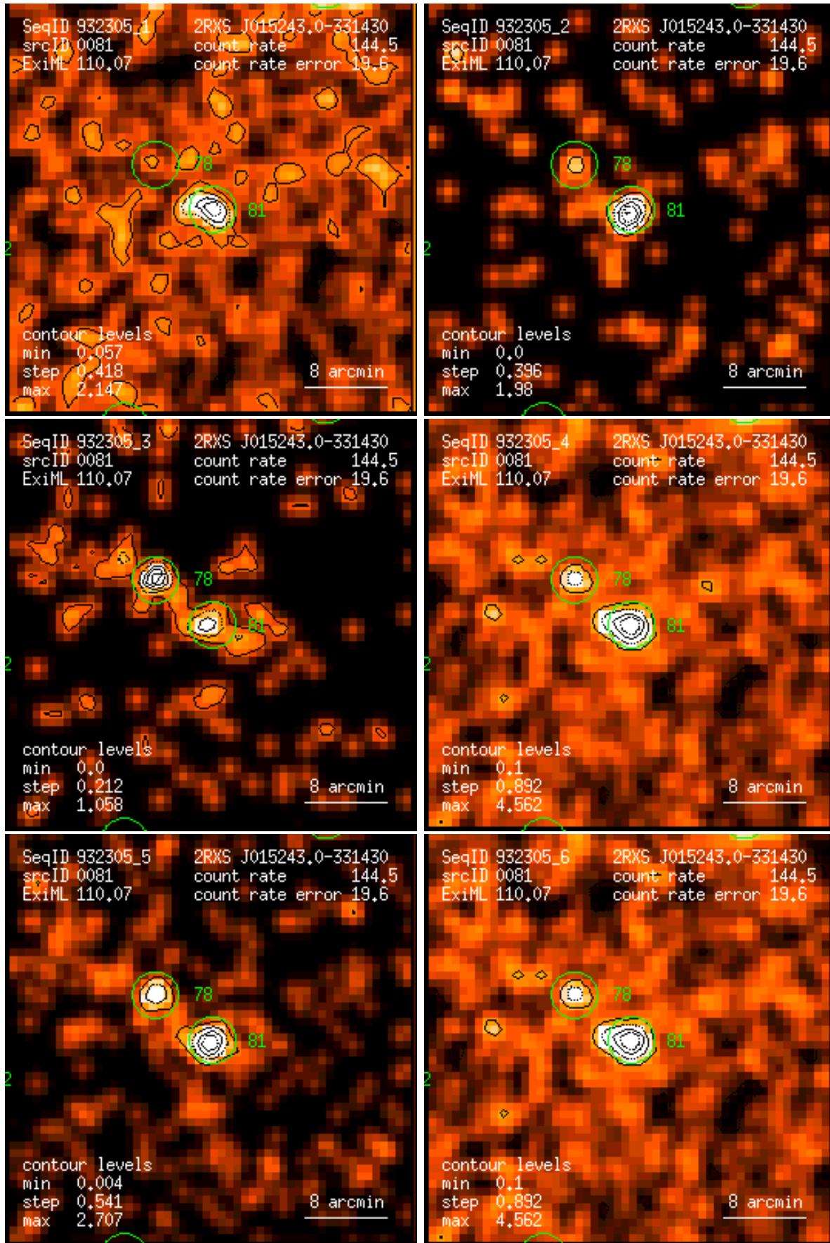
Figure 81: RASS 932305: detection 0081: band rate images, Gaussian filter: (1) PSPC channels 11 – 41, (2) 52 – 90, (3) 91 – 201, (4) 11 – 235, (5) 52 – 201, (6) 11 – 201. Broad band rates in counts/ks. Band rate contour levels in counts/ks/arcmin 2 .
