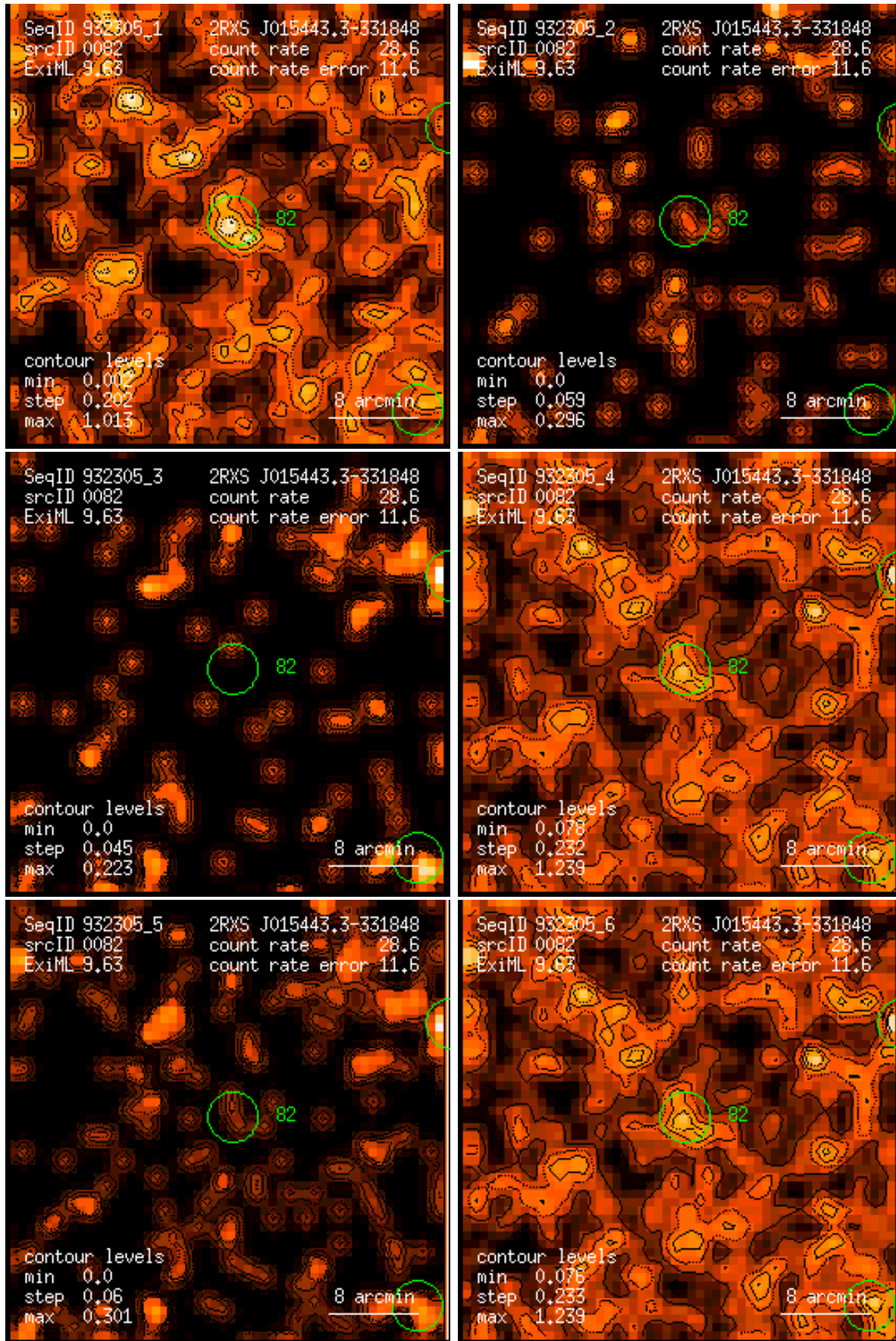
Figure 82: RASS 932305: detection 0082: band rate images, Gaussian filter: (1) PSPC channels 11 – 41, (2) 52 – 90, (3) 91 – 201, (4) 11 – 235, (5) 52 – 201, (6) 11 – 201. Broad band rates in counts/ks. Band rate contour levels in counts/ks/arcmin 2 .
