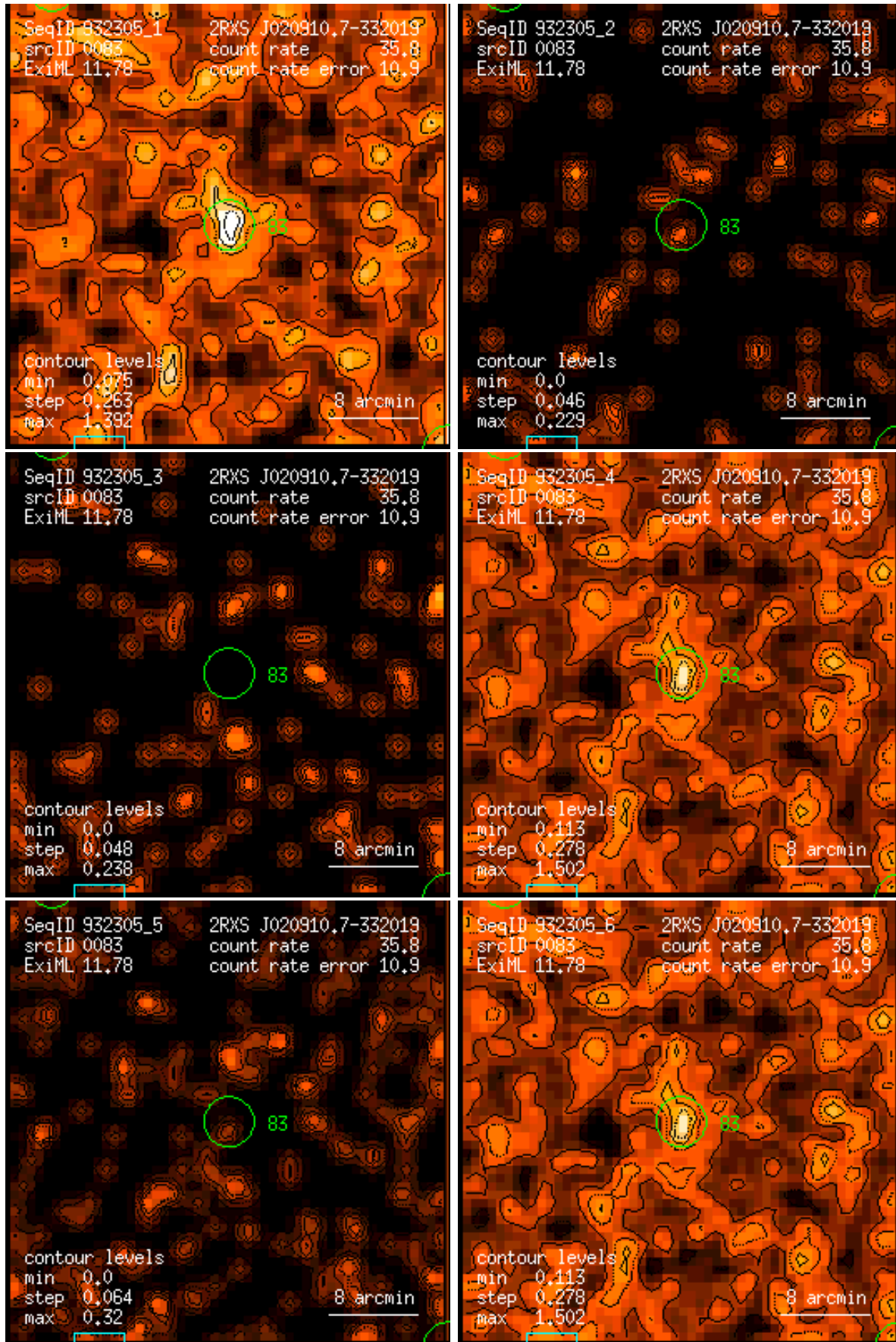
Figure 83: RASS 932305: detection 0083: band rate images, Gaussian filter: (1) PSPC channels 11 – 41, (2) 52 – 90, (3) 91 – 201, (4) 11 – 235, (5) 52 – 201, (6) 11 – 201. Broad band rates in counts/ks. Band rate contour levels in counts/ks/arcmin 2 .
