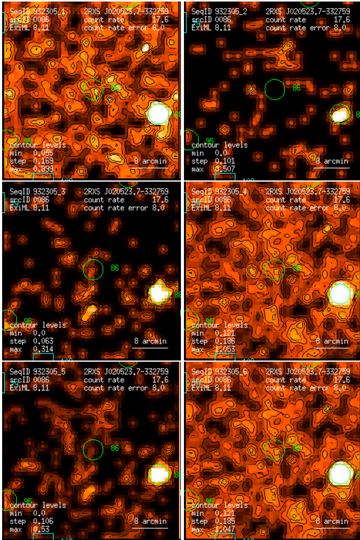
Figure 86: RASS 932305: detection 0086: band rate images, Gaussian filter: (1) PSPC channels 11 – 41, (2) 52 – 90, (3) 91 – 201, (4) 11 – 235, (5) 52 – 201, (6) 11 – 201. Broad band rates in counts/ks. Band rate contour levels in counts/ks/arcmin 2 .
