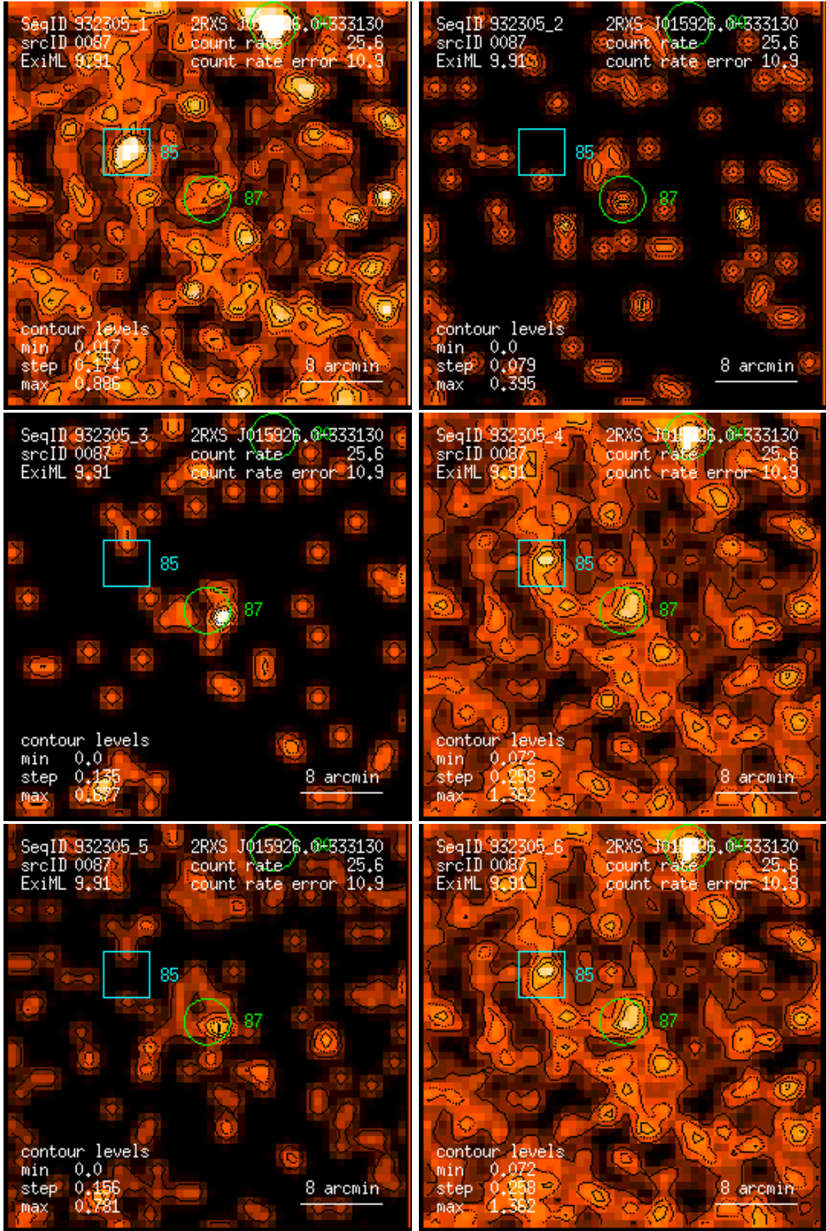
Figure 87: RASS 932305: detection 0087: band rate images, Gaussian filter: (1) PSPC channels 11 – 41, (2) 52 – 90, (3) 91 – 201, (4) 11 – 235, (5) 52 – 201, (6) 11 – 201. Broad band rates in counts/ks. Band rate contour levels in counts/ks/arcmin 2 .
