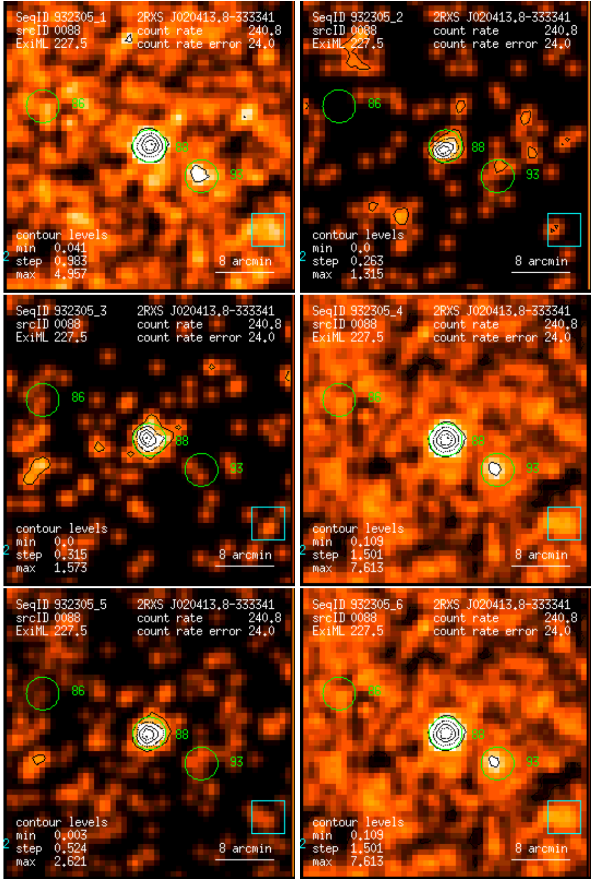
Figure 88: RASS 932305: detection 0088: band rate images, Gaussian filter: (1) PSPC channels 11 – 41, (2) 52 – 90, (3) 91 – 201, (4) 11 – 235, (5) 52 – 201, (6) 11 – 201. Broad band rates in counts/ks. Band rate contour levels in counts/ks/arcmin 2 .
