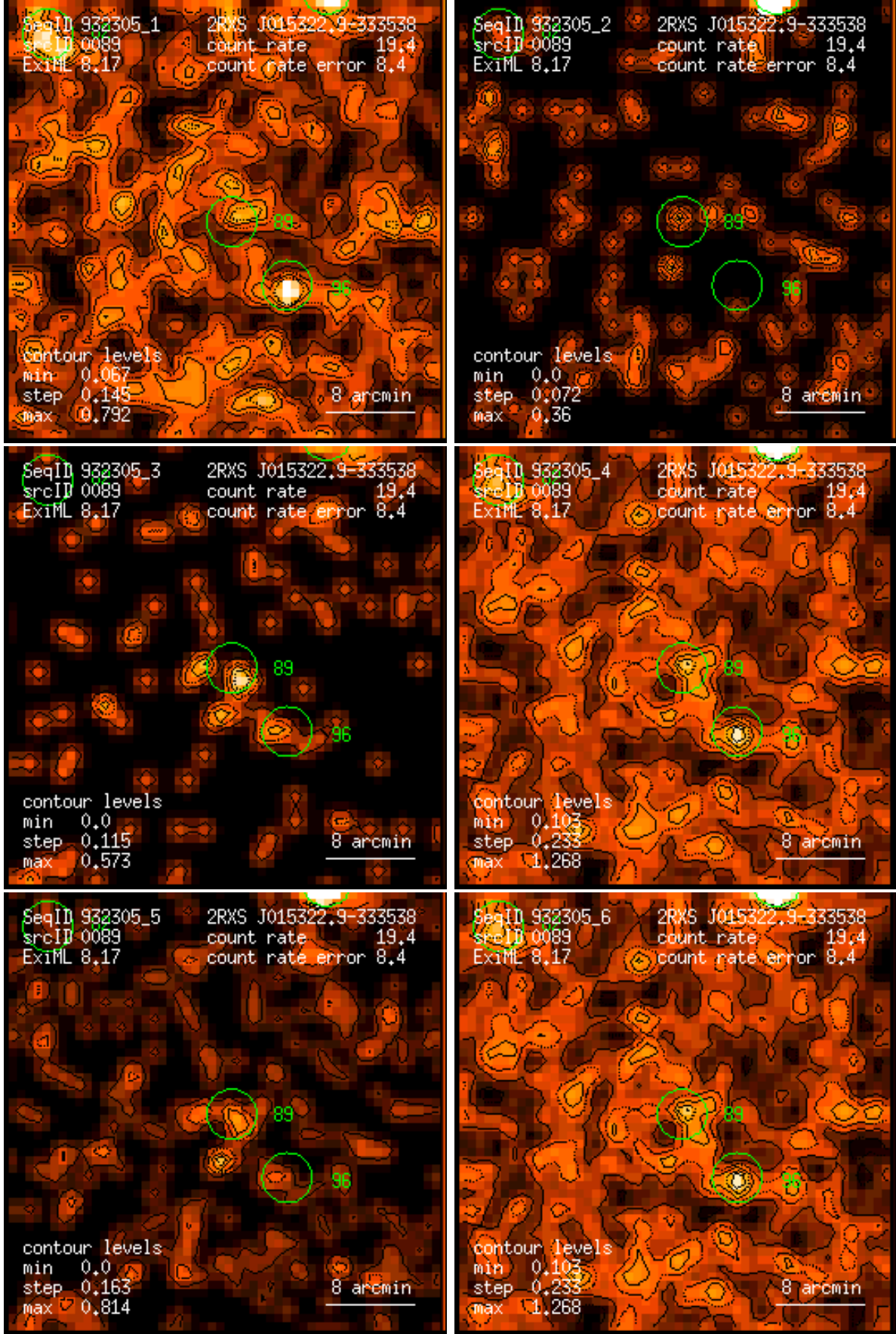
Figure 89: RASS 932305: detection 0089: band rate images, Gaussian filter: (1) PSPC channels 11 – 41, (2) 52 – 90, (3) 91 – 201, (4) 11 – 235, (5) 52 – 201, (6) 11 – 201. Broad band rates in counts/ks. Band rate contour levels in counts/ks/arcmin 2 .
