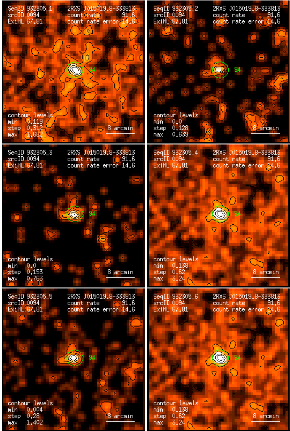
Figure 94: RASS 932305: detection 0094: band rate images, Gaussian filter: (1) PSPC channels 11 – 41, (2) 52 – 90, (3) 91 – 201, (4) 11 – 235, (5) 52 – 201, (6) 11 – 201. Broad band rates in counts/ks. Band rate contour levels in counts/ks/arcmin 2 .
