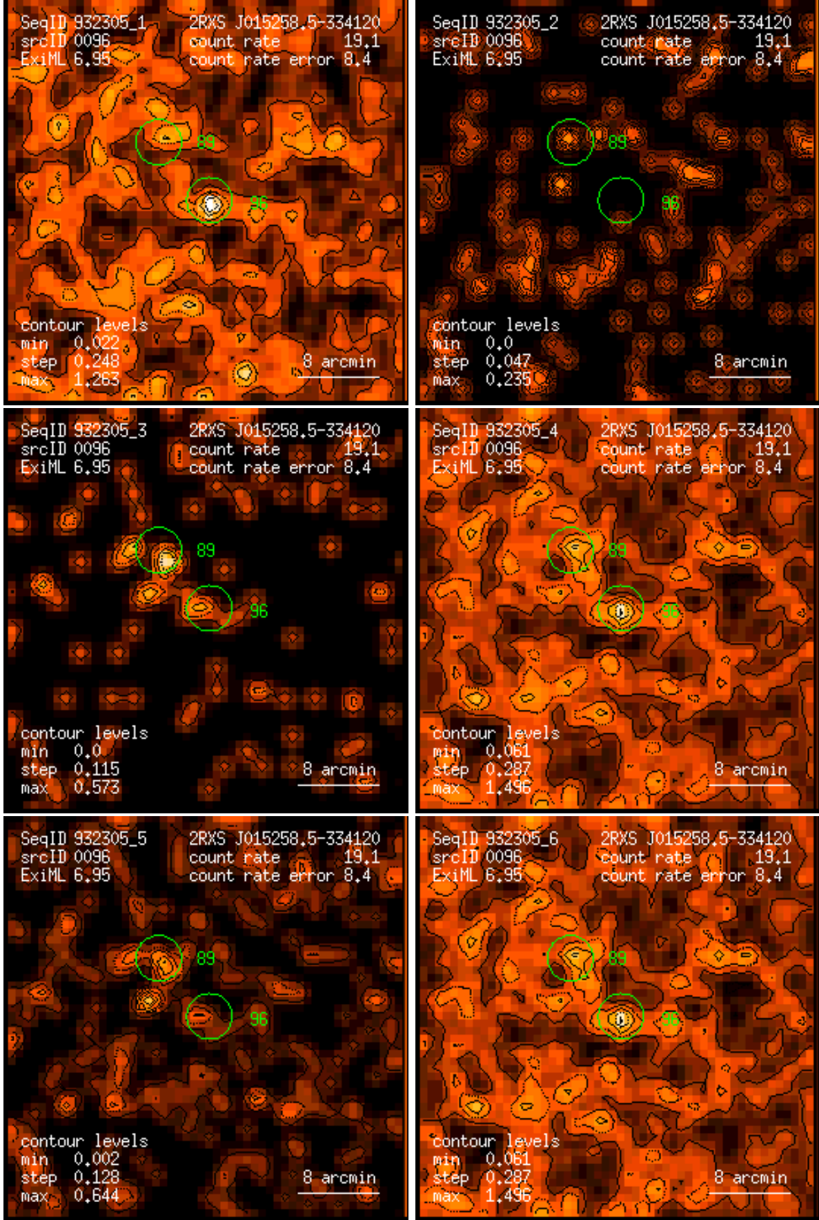
Figure 96: RASS 932305: detection 0096: band rate images, Gaussian filter: (1) PSPC channels 11 – 41, (2) 52 – 90, (3) 91 – 201, (4) 11 – 235, (5) 52 – 201, (6) 11 – 201. Broad band rates in counts/ks. Band rate contour levels in counts/ks/arcmin 2 .
