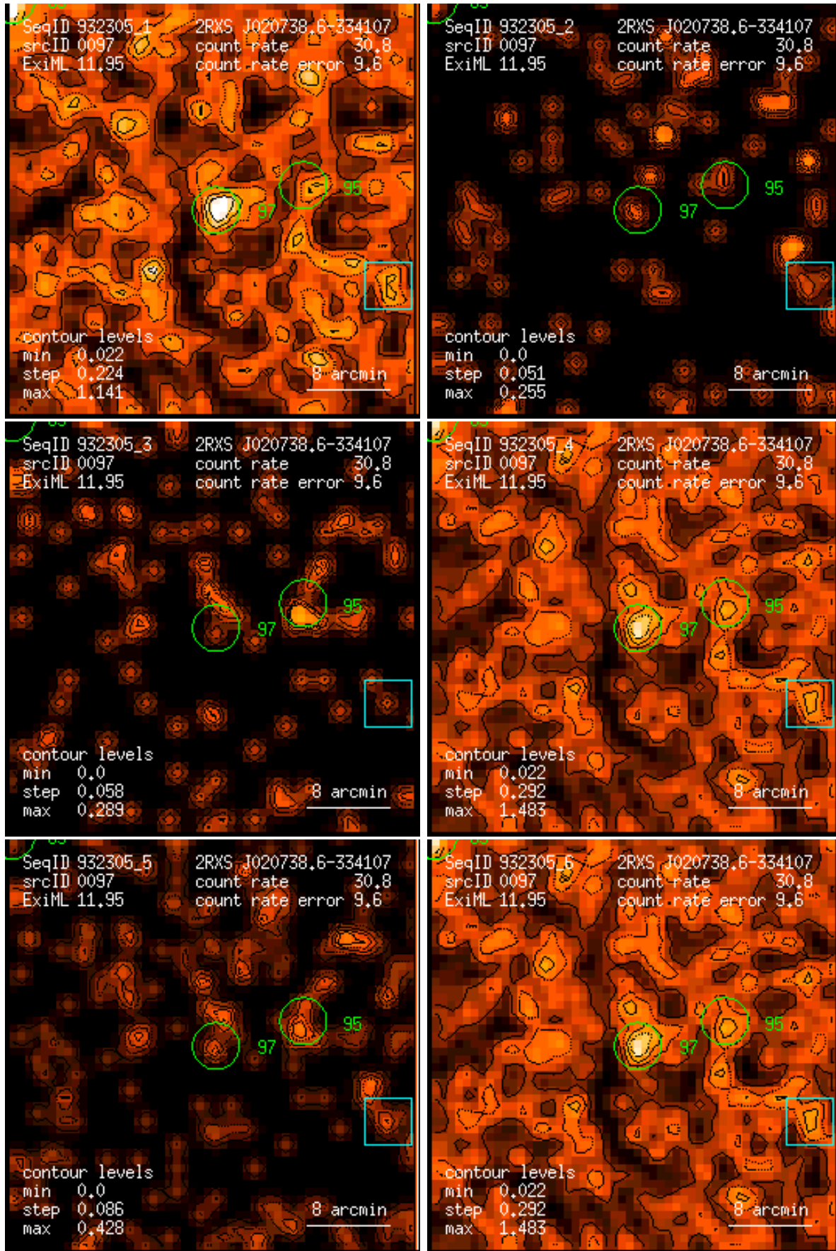
Figure 97: RASS 932305: detection 0097: band rate images, Gaussian filter: (1) PSPC channels 11 – 41, (2) 52 – 90, (3) 91 – 201, (4) 11 – 235, (5) 52 – 201, (6) 11 – 201. Broad band rates in counts/ks. Band rate contour levels in counts/ks/arcmin 2 .
