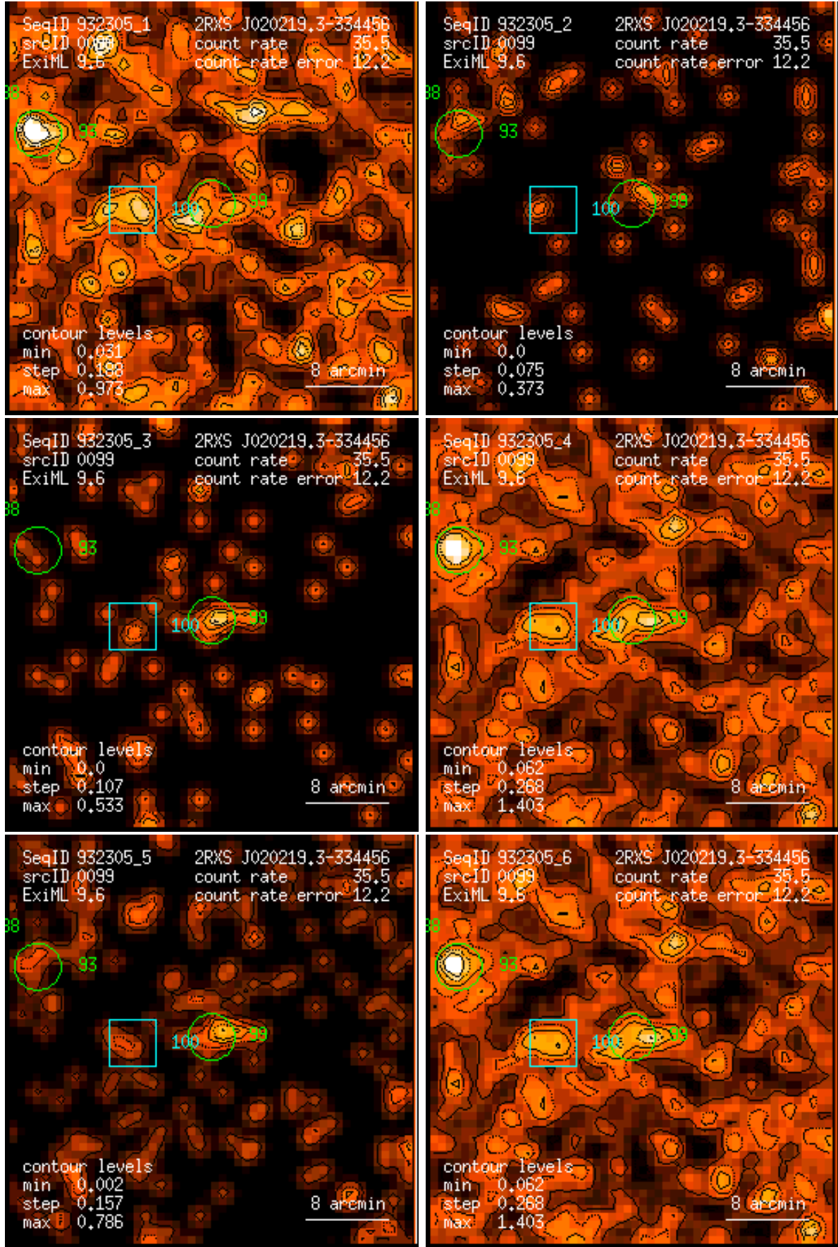
Figure 99: RASS 932305: detection 0099: band rate images, Gaussian filter: (1) PSPC channels 11 – 41, (2) 52 – 90, (3) 91 – 201, (4) 11 – 235, (5) 52 – 201, (6) 11 – 201. Broad band rates in counts/ks. Band rate contour levels in counts/ks/arcmin 2 .
