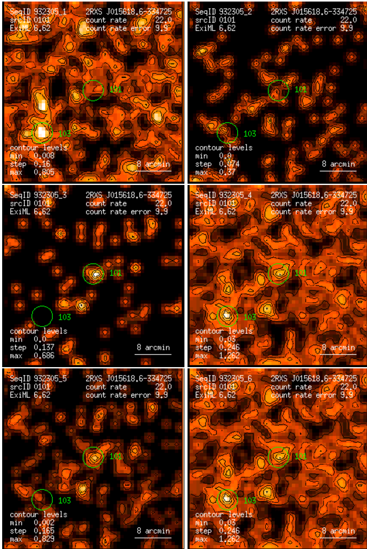
Figure 101: RASS 932305: detection 0101: band rate images, Gaussian filter: (1) PSPC channels 11 – 41, (2) 52 – 90, (3) 91 – 201, (4) 11 – 235, (5) 52 – 201, (6) 11 – 201. Broad band rates in counts/ks. Band rate contour levels in counts/ks/arcmin 2 .
