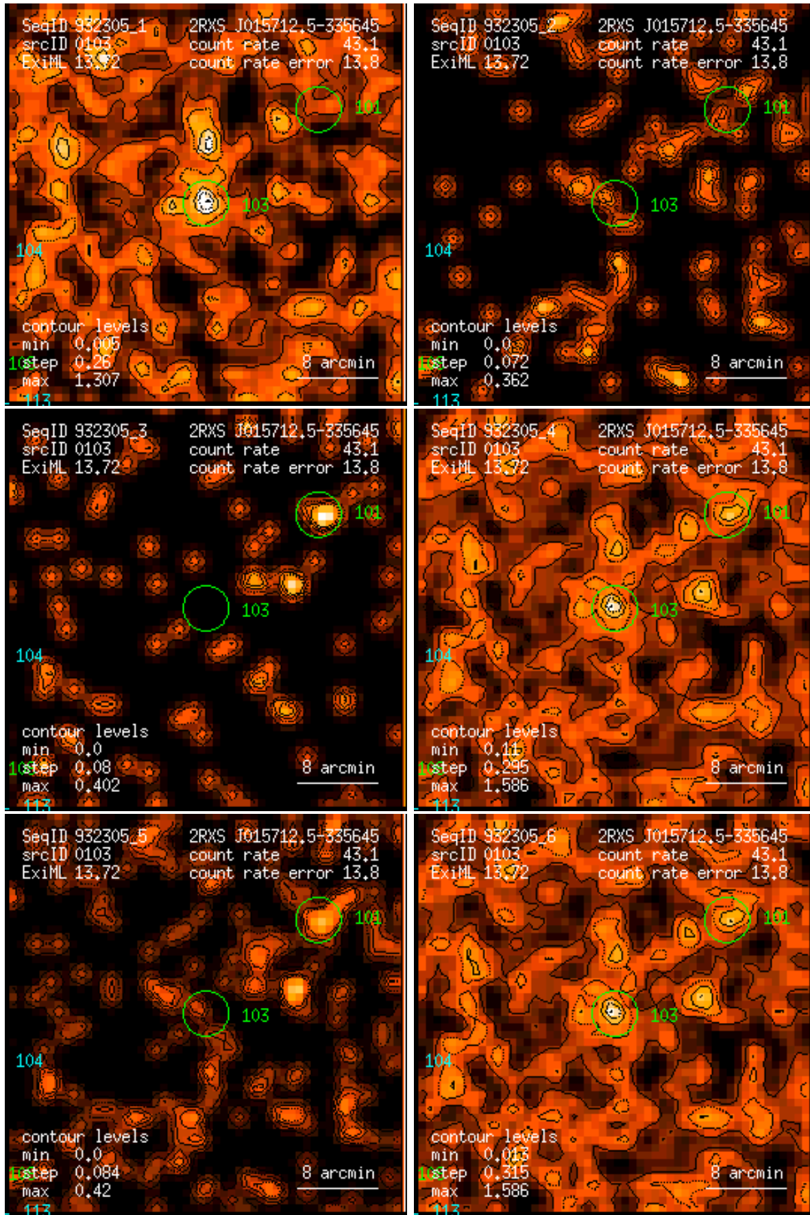
Figure 103: RASS 932305: detection 0103: band rate images, Gaussian filter: (1) PSPC channels 11 – 41, (2) 52 – 90, (3) 91 – 201, (4) 11 – 235, (5) 52 – 201, (6) 11 – 201. Broad band rates in counts/ks. Band rate contour levels in counts/ks/arcmin 2 .
