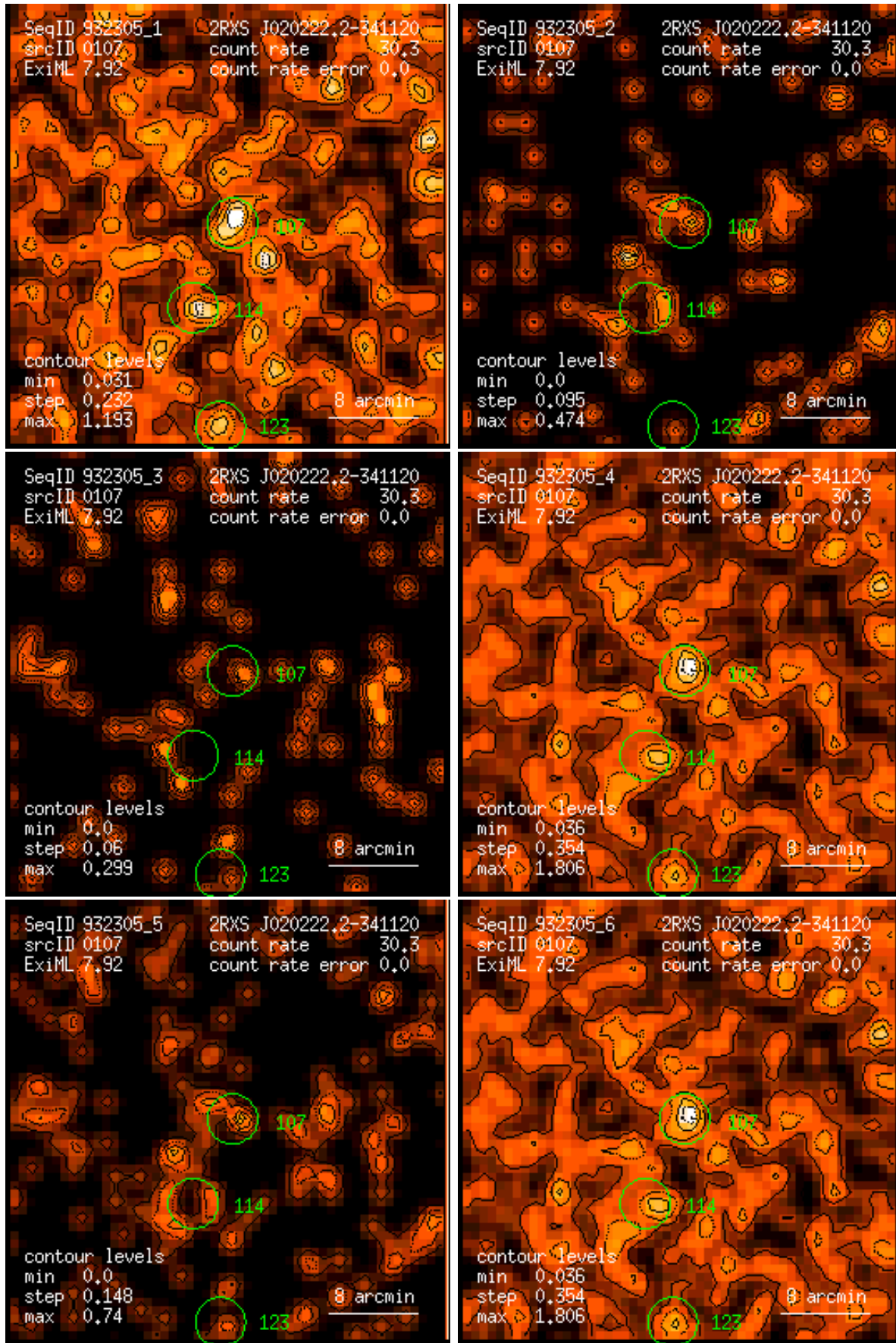
Figure 107: RASS 932305: detection 0107: band rate images, Gaussian filter: (1) PSPC channels 11 – 41, (2) 52 – 90, (3) 91 – 201, (4) 11 – 235, (5) 52 – 201, (6) 11 – 201. Broad band rates in counts/ks. Band rate contour levels in counts/ks/arcmin 2 .
